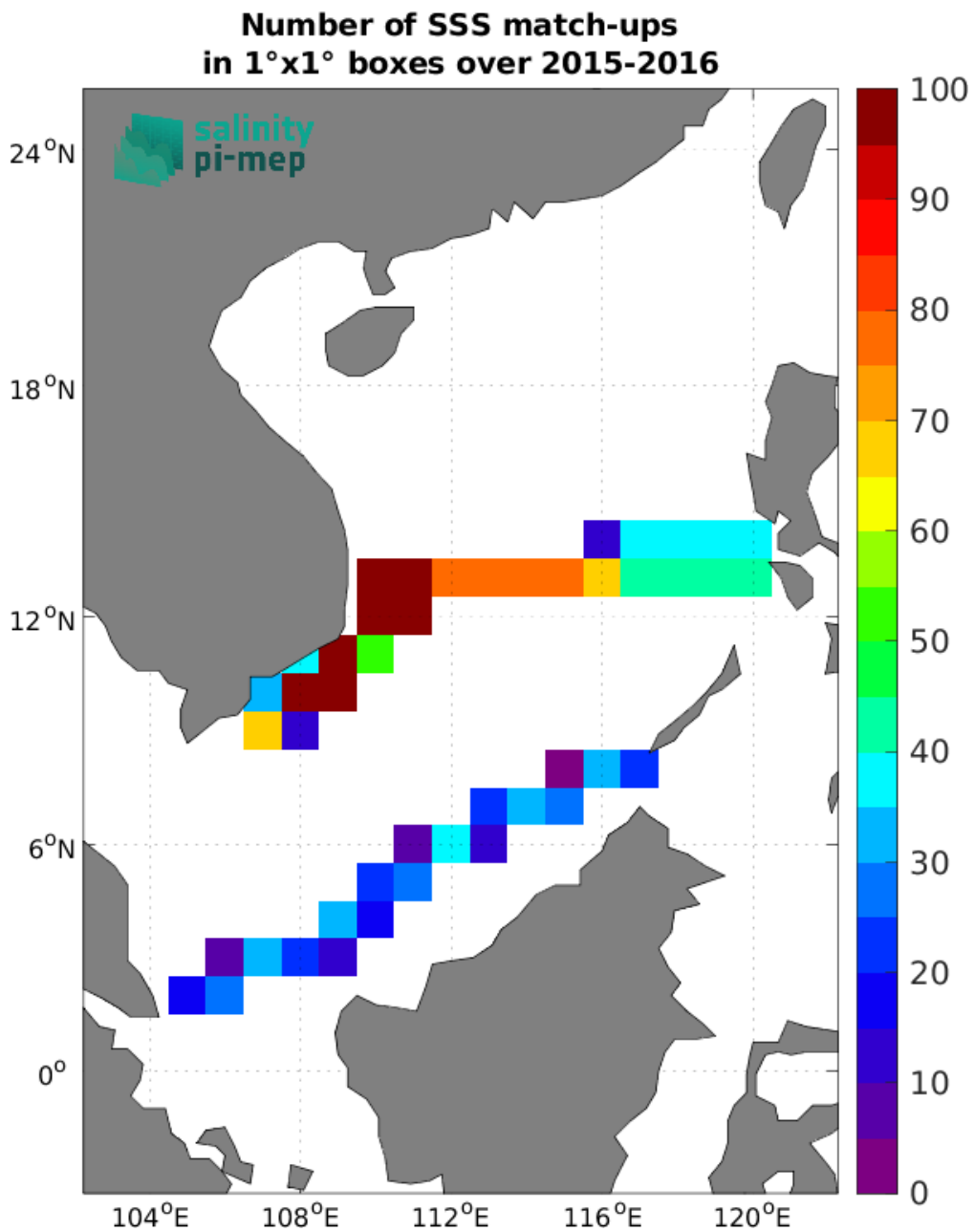
Figure 5: Number of SSS match-ups between TSG (SAMOS) SSS and the SMAP SSS L3 v6 - 8-Day running (RSS) SSS product for the South China Sea Pi-MEP region over 1°x1° boxes and for the full satellite product period.
