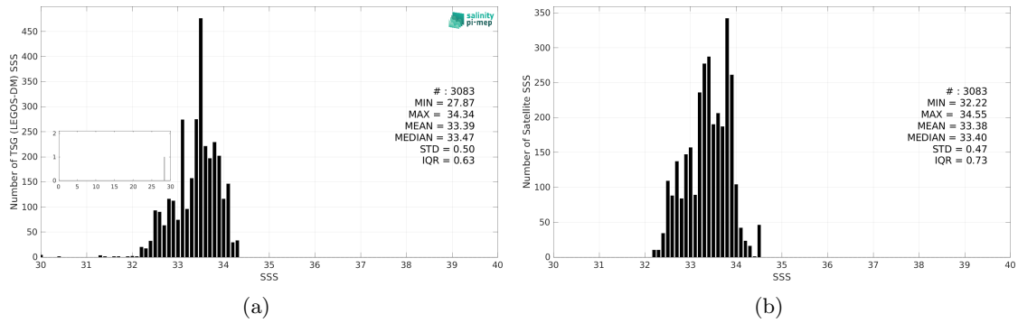
Figure 3: Histograms of SSS from TSG (LEGOS-DM) (a) and SMAP SSS L3 v6 - 8-Day running (RSS) (b) considering all match-up pairs per bins of 0.1 over the South China Sea Pi-MEP region and for the full satellite product period.
