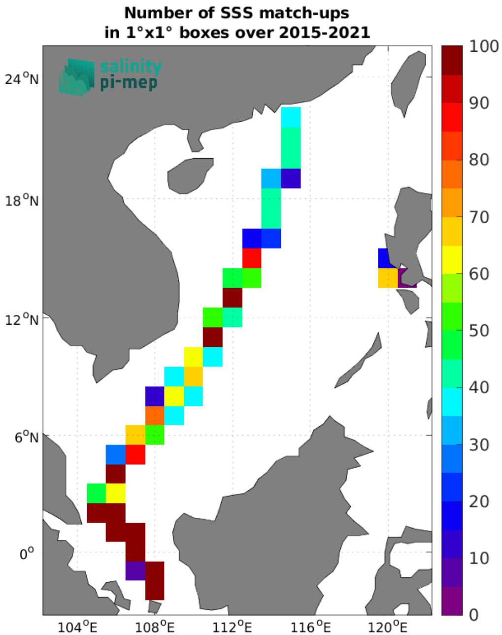
Figure 5: Number of SSS match-ups between TSG (LEGOS-DM) SSS and the SMAP SSS L3 v6 - 8-Day running (RSS) SSS product for the South China Sea Pi-MEP region over 1^\circ \times 1^\circ boxes and for the full satellite product period.
