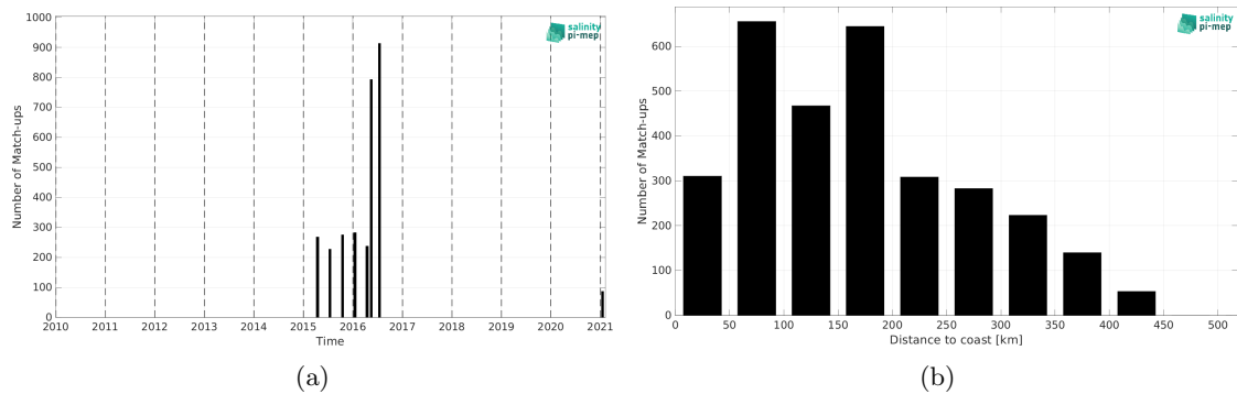
Figure 2: Number of match-ups between TSG (LEGOS-DM) and SMAP SSS L3 v6 - 8-Day running (RSS) SSS as a function of time (a) and as function of the distance to coast (b) over the South China Sea Pi-MEP region and for the full satellite product period.
