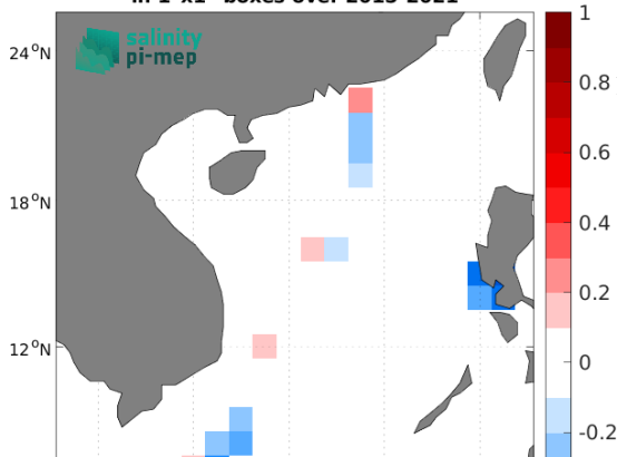
Temporal mean of (Sat - TSG (LEGOS-DM)) in 1°x1° boxes over 2015-2021
