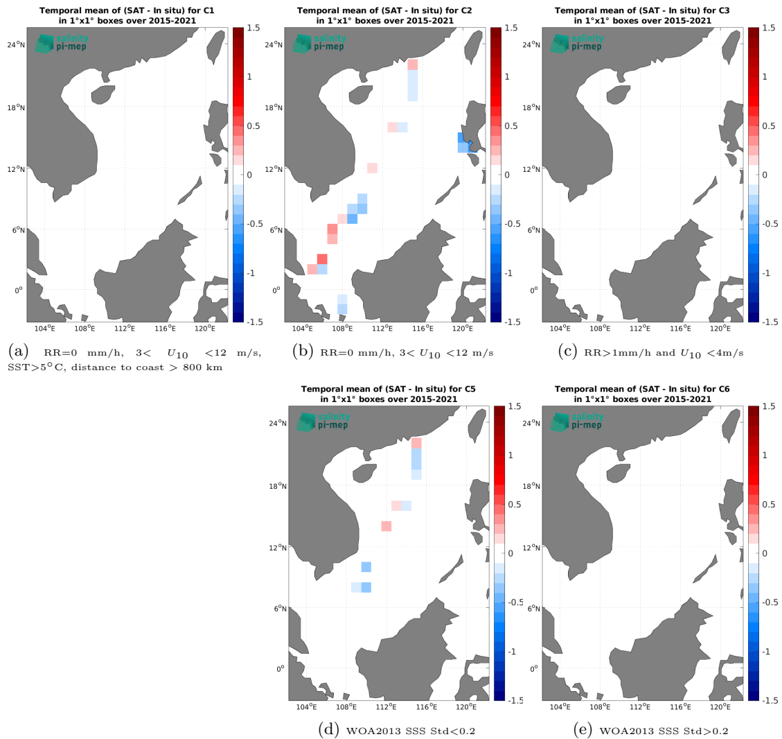
Figure 14: Temporal mean gridded over spatial boxes of size 1^\circ \times 1^\circ of \Delta\text{SSS} (SMAP SSS L3 v6 - 8-Day running (RSS) - TSG (LEGOS-DM)) for 5 different subdatasets corresponding to: RR=0 mm/h, 3 < U_{10} < 12 m/s, SST > 5^\circ\text{C} , distance to coast > 800 km (a), RR=0 mm/h, 3 < U_{10} < 12 m/s (b), RR > 1 mm/h and U_{10} < 4 m/s (c), WOA2013 SSS Std < 0.2 (d), WOA2013 SSS Std > 0.2 (e).
