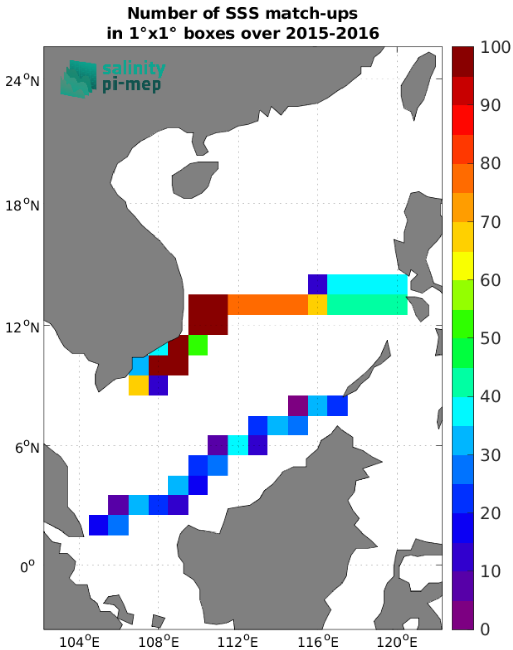
Figure 5: Number of SSS match-ups between TSG (SAMOS) SSS and the SMAP SSS L3 v6 - Monthly (RSS) SSS product for the South China Sea Pi-MEP region over 1^{\circ} \times 1^{\circ} boxes and for the full satellite product period.
