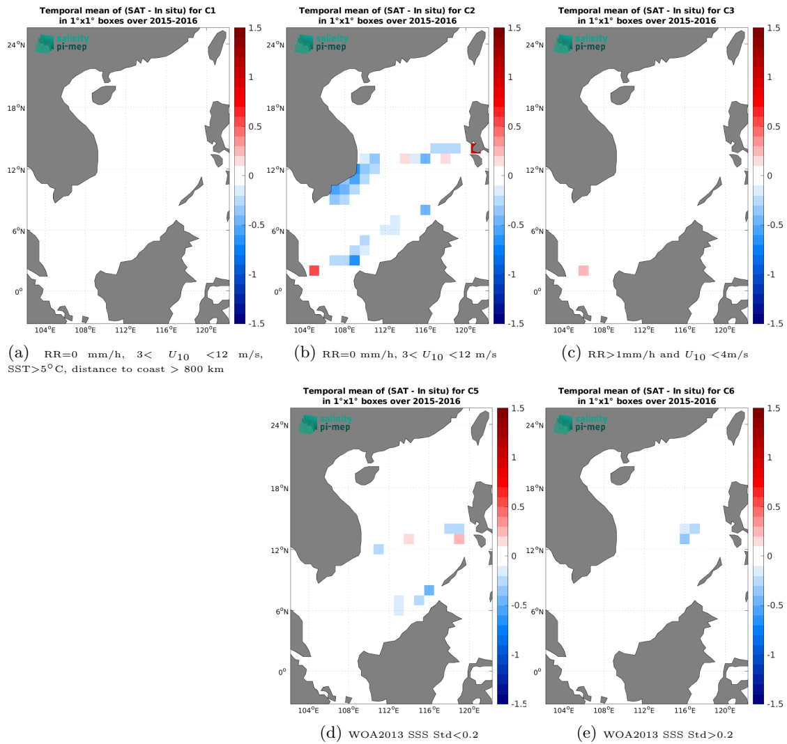
Figure 14: Temporal mean gridded over spatial boxes of size 1^\circ \times 1^\circ of \Delta\text{SSS} (SMAP SSS L3 v6 - Monthly (RSS) - TSG (SAMOS)) for 5 different subdatasets corresponding to: RR=0 mm/h, 3 < U_{10} < 12 m/s, SST > 5^\circ\text{C} , distance to coast > 800 km (a), RR=0 mm/h, 3 < U_{10} < 12 m/s (b), RR > 1 mm/h and U_{10} < 4 m/s (c), WOA2013 SSS Std < 0.2 (d), WOA2013 SSS Std > 0.2 (e).
