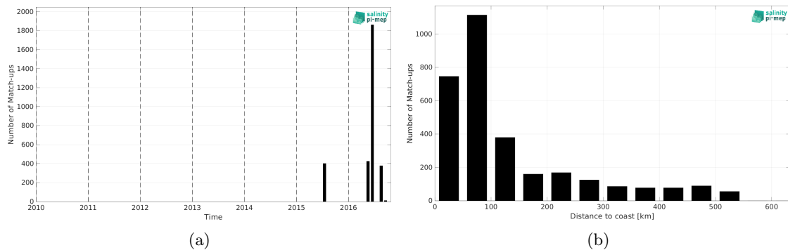
Figure 2: Number of match-ups between TSG (SAMOS) and SMAP SSS L3 v6 - Monthly (RSS) SSS as a function of time (a) and as function of the distance to coast (b) over the South China Sea Pi-MEP region and for the full satellite product period.
