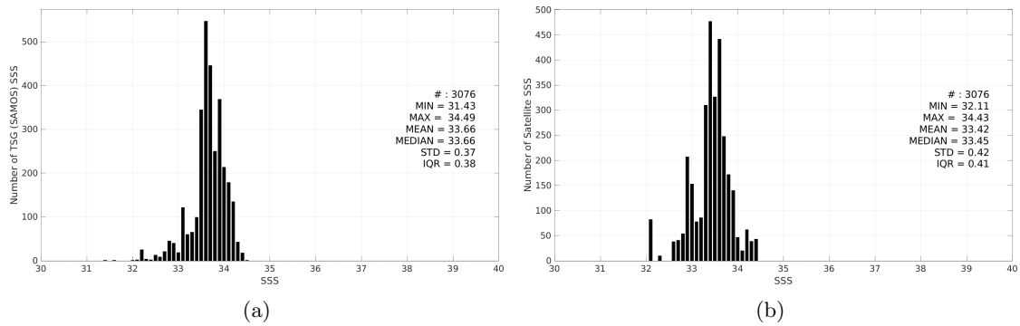
Figure 3: Histograms of SSS from TSG (SAMOS) (a) and SMAP SSS L3 v6 - Monthly (RSS) (b) considering all match-up pairs per bins of 0.1 over the South China Sea Pi-MEP region and for the full satellite product period.
