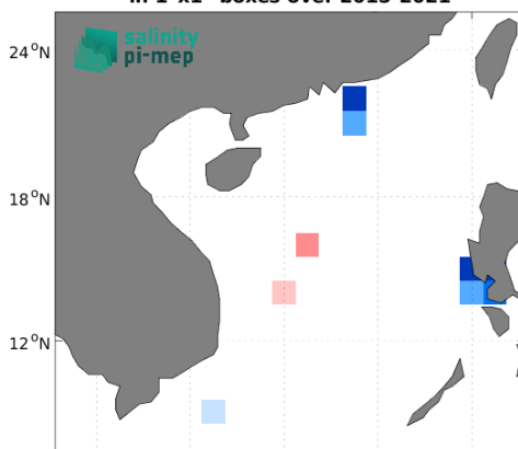
Temporal mean of (Sat - TSG (LEGOS-DM)) in 1°x1° boxes over 2015-2021
