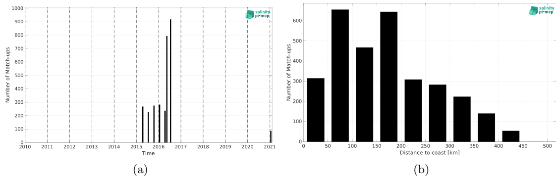
Figure 2: Number of match-ups between TSG (LEGOS-DM) and SMAP SSS L3 v6 - Monthly (RSS) SSS as a function of time (a) and as function of the distance to coast (b) over the South China Sea Pi-MEP region and for the full satellite product period.
