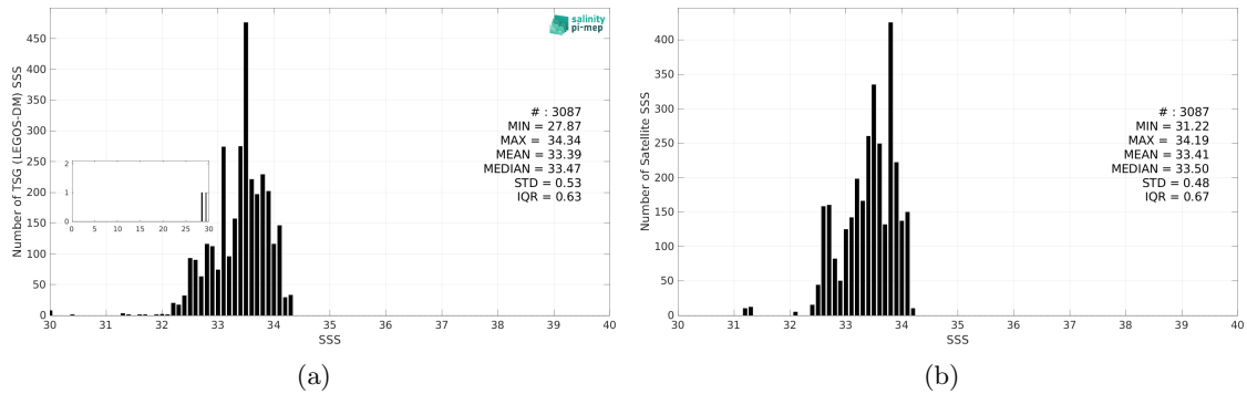
Figure 3: Histograms of SSS from TSG (LEGOS-DM) (a) and SMAP SSS L3 v6 - Monthly (RSS) (b) considering all match-up pairs per bins of 0.1 over the South China Sea Pi-MEP region and for the full satellite product period.
