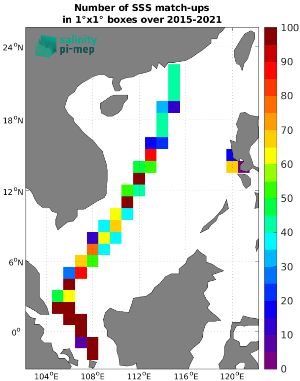
Figure 5: Number of SSS match-ups between TSG (LEGOS-DM) SSS and the SMAP SSS L3 v6 - Monthly (RSS) SSS product for the South China Sea Pi-MEP region over 1°x1° boxes and for the full satellite product period.
