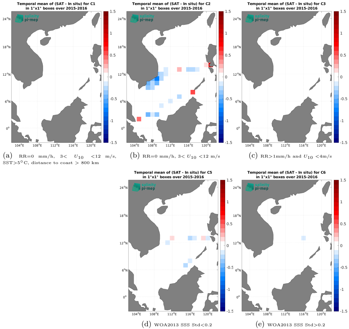
Figure 14: Temporal mean gridded over spatial boxes of size 1^\circ \times 1^\circ of \Delta\text{SSS} (SMAP SSS L3 v5.3 - 8-Day running (RSS) - TSG (SAMOS)) for 5 different subdatasets corresponding to: RR=0 mm/h, 3 < U_{10} < 12 m/s, SST > 5^\circ\text{C} , distance to coast > 800 km (a), RR=0 mm/h, 3 < U_{10} < 12 m/s (b), RR > 1 mm/h and U_{10} < 4 m/s (c), WOA2013 SSS Std < 0.2 (d), WOA2013 SSS Std > 0.2 (e).
