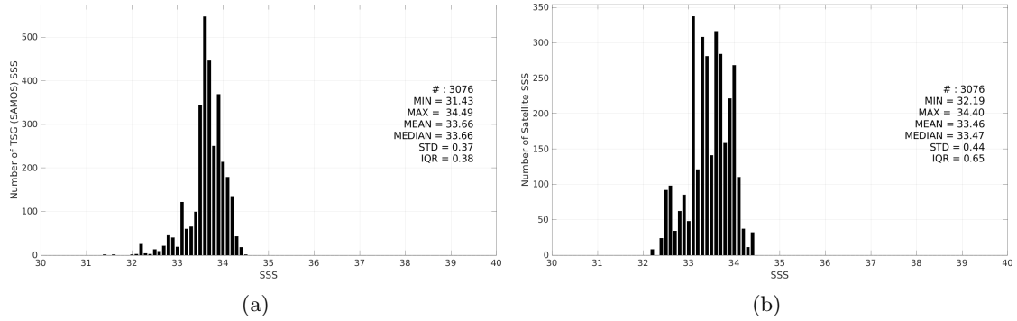
Figure 3: Histograms of SSS from TSG (SAMOS) (a) and SMAP SSS L3 v5.3 - 8-Day running (RSS) (b) considering all match-up pairs per bins of 0.1 over the South China Sea Pi-MEP region and for the full satellite product period.
