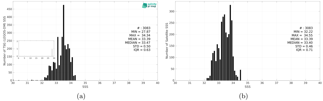
Figure 3: Histograms of SSS from TSG (LEGOS-DM) (a) and SMAP SSS L3 v5.3 - 8-Day running (RSS) (b) considering all match-up pairs per bins of 0.1 over the South China Sea Pi-MEP region and for the full satellite product period.
