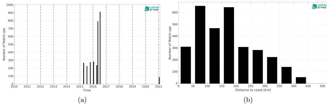
Figure 2: Number of match-ups between TSG (LEGOS-DM) and SMAP SSS L3 v5.3 - 8-Day running (RSS) SSS as a function of time (a) and as function of the distance to coast (b) over the South China Sea Pi-MEP region and for the full satellite product period.
