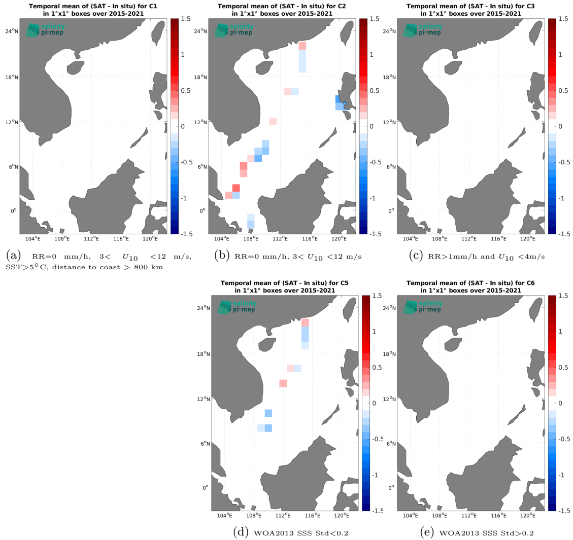
Figure 14: Temporal mean gridded over spatial boxes of size 1^\circ \times 1^\circ of \Delta\text{SSS} (SMAP SSS L3 v5.3 - 8-Day running (RSS) - TSG (LEGOS-DM)) for 5 different subdatasets corresponding to: RR=0 mm/h, 3 < U_{10} < 12 m/s, SST > 5^\circ\text{C} , distance to coast > 800 km (a), RR=0 mm/h, 3 < U_{10} < 12 m/s (b), RR > 1 mm/h and U_{10} < 4 m/s (c), WOA2013 SSS Std < 0.2 (d), WOA2013 SSS Std > 0.2 (e).
