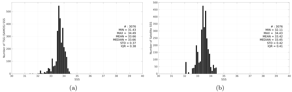
Figure 3: Histograms of SSS from TSG (SAMOS) (a) and SMAP SSS L3 v5.3 - Monthly (RSS) (b) considering all match-up pairs per bins of 0.1 over the South China Sea Pi-MEP region and for the full satellite product period.
