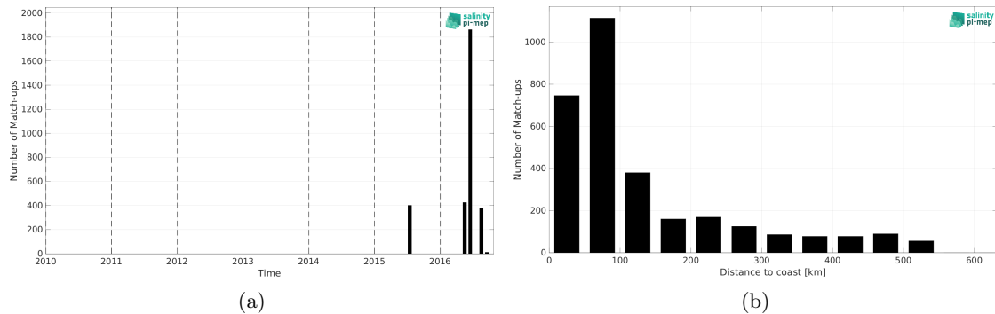
Figure 2: Number of match-ups between TSG (SAMOS) and SMAP SSS L3 v5.3 - Monthly (RSS) SSS as a function of time (a) and as function of the distance to coast (b) over the South China Sea Pi-MEP region and for the full satellite product period.
