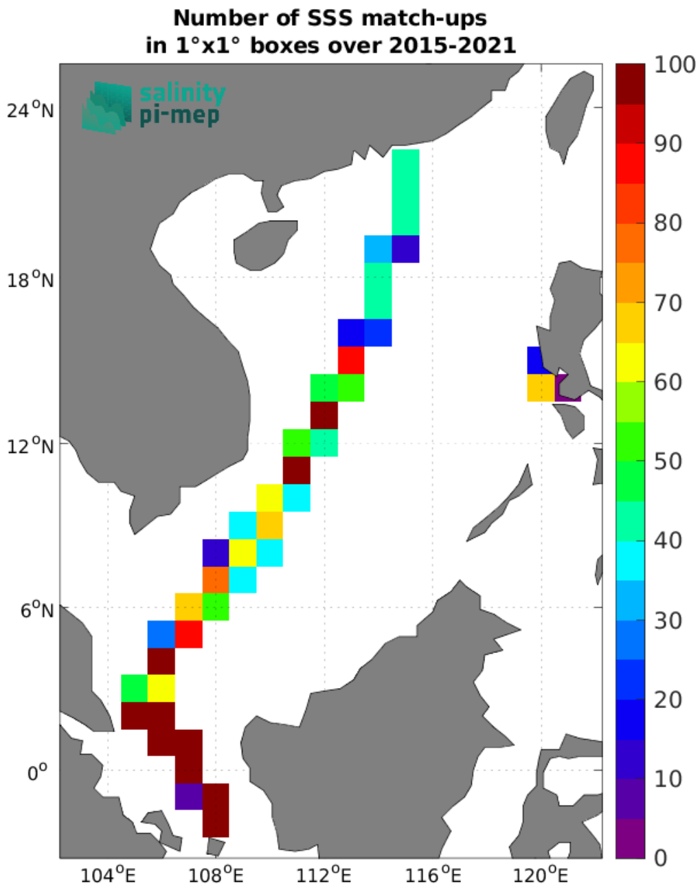
Figure 5: Number of SSS match-ups between TSG (LEGOS-DM) SSS and the SMAP SSS L3 v5.3 - Monthly (RSS) SSS product for the South China Sea Pi-MEP region over 1^{\circ} \times 1^{\circ} boxes and for the full satellite product period.
