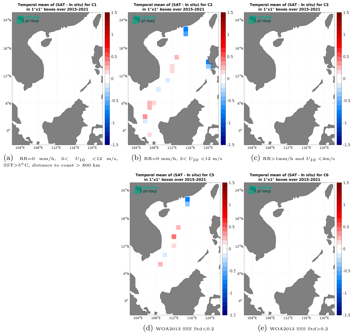
Figure 14: Temporal mean gridded over spatial boxes of size 1^\circ \times 1^\circ of \Delta\text{SSS} (SMAP SSS L3 v5.3 - Monthly (RSS) - TSG (LEGOS-DM)) for 5 different subdatasets corresponding to: RR=0 mm/h, 3 < U_{10} < 12 m/s, SST > 5^\circ\text{C} , distance to coast > 800 km (a), RR=0 mm/h, 3 < U_{10} < 12 m/s (b), RR > 1 mm/h and U_{10} < 4 m/s (c), WOA2013 SSS Std < 0.2 (d), WOA2013 SSS Std > 0.2 (e).
