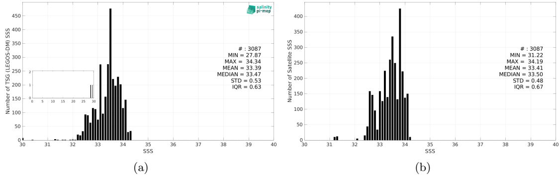
Figure 3: Histograms of SSS from TSG (LEGOS-DM) (a) and SMAP SSS L3 v5.3 - Monthly (RSS) (b) considering all match-up pairs per bins of 0.1 over the South China Sea Pi-MEP region and for the full satellite product period.
