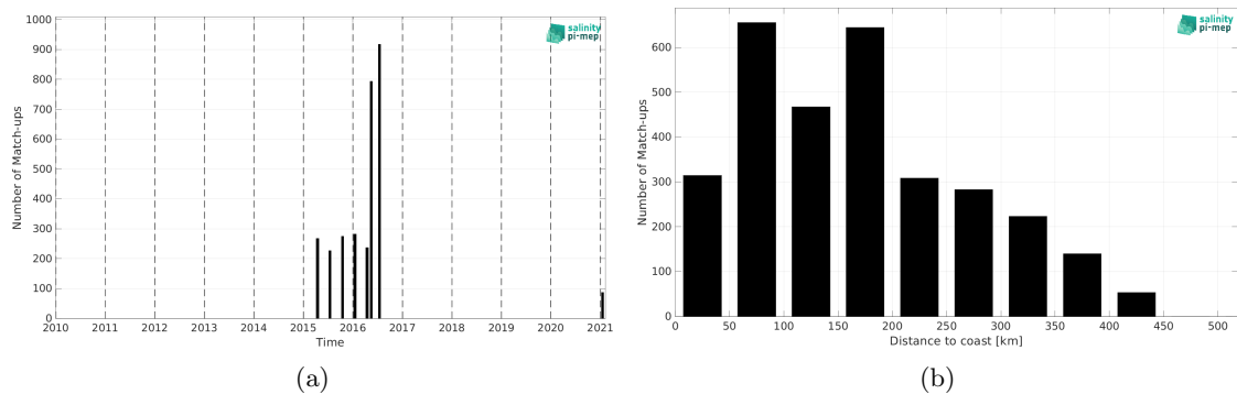
Figure 2: Number of match-ups between TSG (LEGOS-DM) and SMAP SSS L3 v5.3 - Monthly (RSS) SSS as a function of time (a) and as function of the distance to coast (b) over the South China Sea Pi-MEP region and for the full satellite product period.
