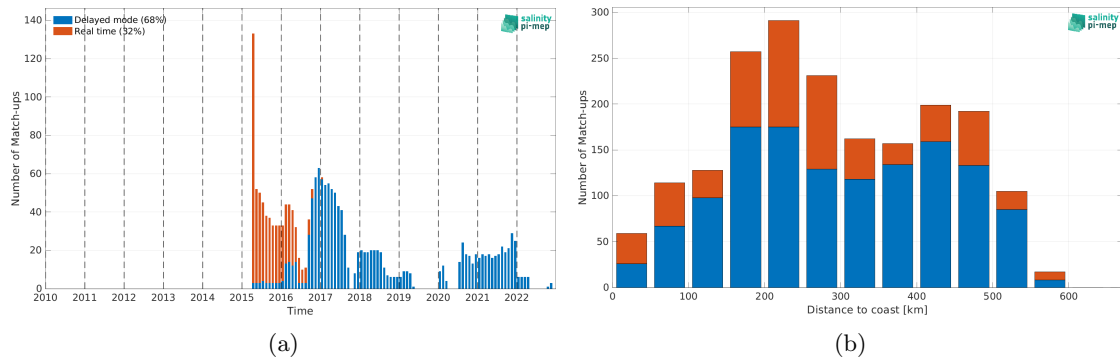
Figure 2: Number of match-ups between Argo and SMAP SSS L3 v5.3 - Monthly (RSS) SSS as a function of time (a) and as function of the distance to coast (b) over the South China Sea Pi-MEP region and for the full satellite product period.
