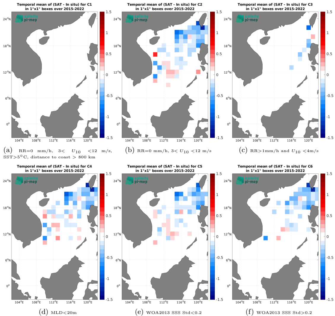
Figure 14: Temporal mean gridded over spatial boxes of size 1^\circ \times 1^\circ of \Delta SSS (SMAP SSS L3 v5.3 - Monthly (RSS) - Argo) for 6 different subdatasets corresponding to: RR=0 mm/h, 3 < U_{10} < 12 m/s, SST > 5°C, distance to coast > 800 km (a), RR=0 mm/h, 3 < U_{10} < 12 m/s (b), RR > 1mm/h and U_{10} < 4 m/s (c), MLD < 20m (d), WOA2013 SSS Std < 0.2 (e), WOA2013 SSS Std > 0.2 (f).
