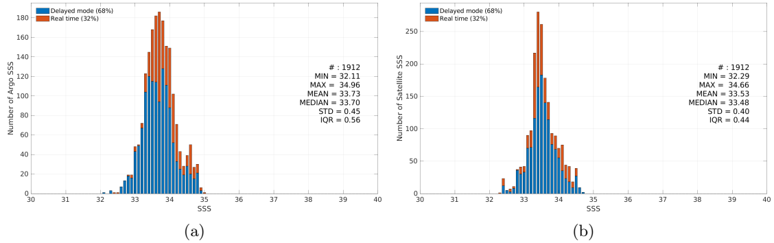
Figure 3: Histograms of SSS from Argo (a) and SMAP SSS L3 v5.3 - Monthly (RSS) (b) considering all match-up pairs per bins of 0.1 over the South China Sea Pi-MEP region and for the full satellite product period.
