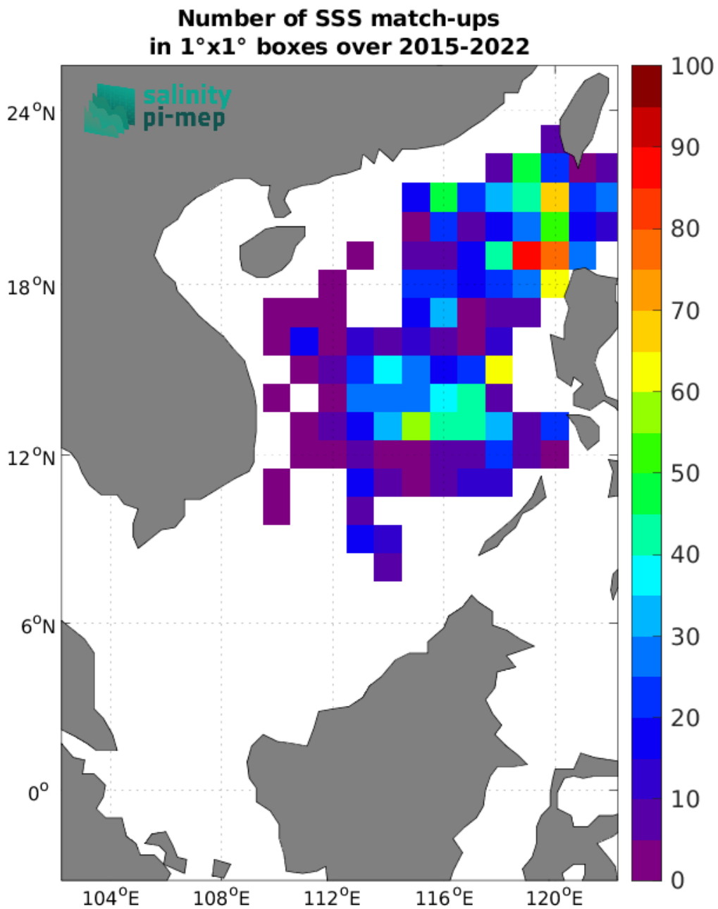
Figure 5: Number of SSS match-ups between Argo SSS and the SMAP SSS L3 v5.3 - Monthly (RSS) SSS product for the South China Sea Pi-MEP region over 1^\circ \times 1^\circ boxes and for the full satellite product period.
