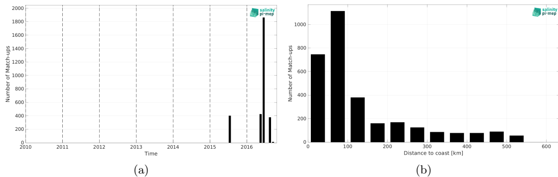
Figure 1: Number of match-ups between TSG (SAMOS) and SMAP SSS L3 v5 - 8-Day running (RSS) SSS as a function of time (a) and as function of the distance to coast (b) over the South China Sea Pi-MEP region and for the full satellite product period.
