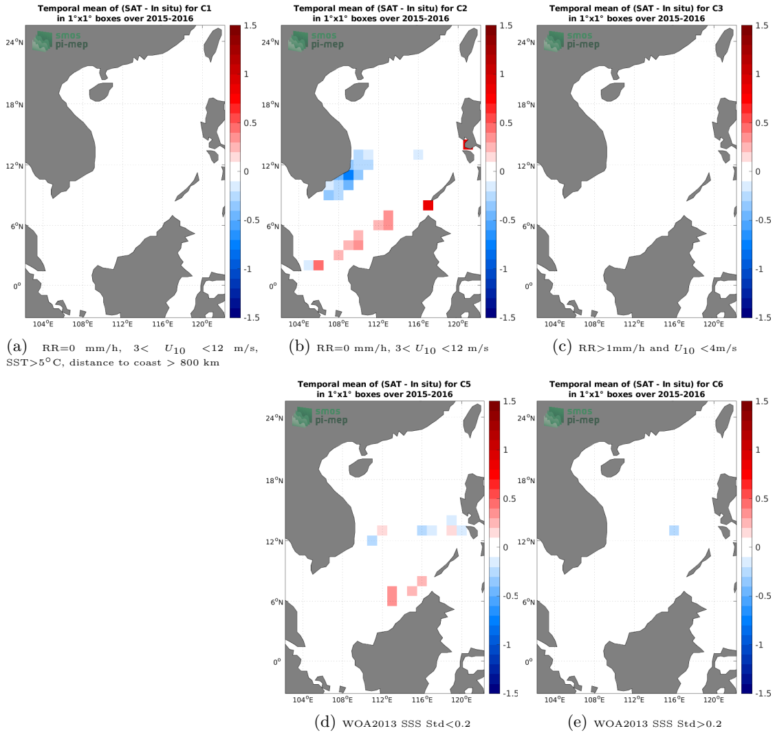
Figure 12: Temporal mean gridded over spatial boxes of size 1^\circ \times 1^\circ of \Delta\text{SSS} (SMAP SSS L3 v5 - 8-Day running (RSS) - TSG (SAMOS)) for 5 different subdatasets corresponding to: RR=0 mm/h, 3 < U_{10} < 12 m/s, SST > 5^\circ\text{C} , distance to coast > 800 km (a), RR=0 mm/h, 3 < U_{10} < 12 m/s (b), RR > 1 mm/h and U_{10} < 4 m/s (c), WOA2013 SSS Std < 0.2 (d), WOA2013 SSS Std > 0.2 (e).
