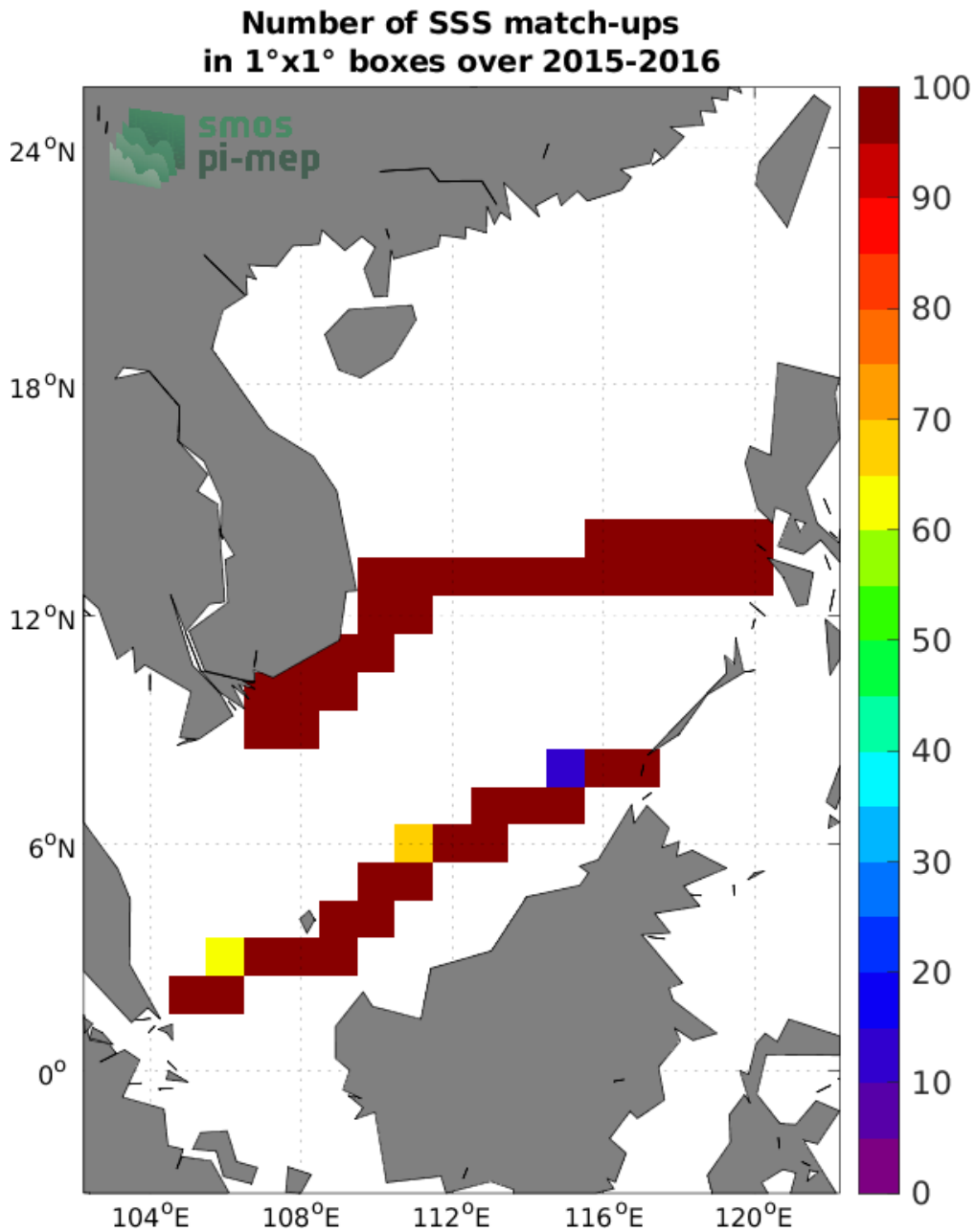
Figure 4: Number of SSS match-ups between TSG (SAMOS) SSS and the SMAP SSS L3 v5 - 8-Day running (RSS) SSS product for the South China Sea Pi-MEP region over 1^\circ \times 1^\circ boxes and for the full satellite product period.
