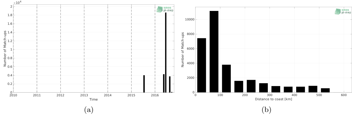
Figure 1: Number of match-ups between TSG (SAMOS) and SMAP SSS L3 v5 - 8-Day running (RSS) SSS as a function of time (a) and as function of the distance to coast (b) over the South China Sea Pi-MEP region and for the full satellite product period.
