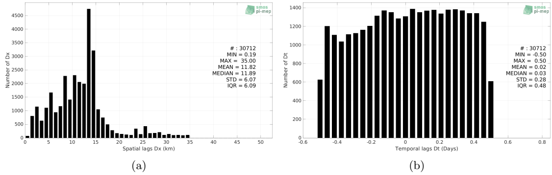
Figure 5: Histograms of the spatial (a) and temporal (b) lags between the location/time of the TSG (SAMOS) measurement and the date of the corresponding SMAP SSS L3 v5 - 8-Day running (RSS) SSS pixel.
