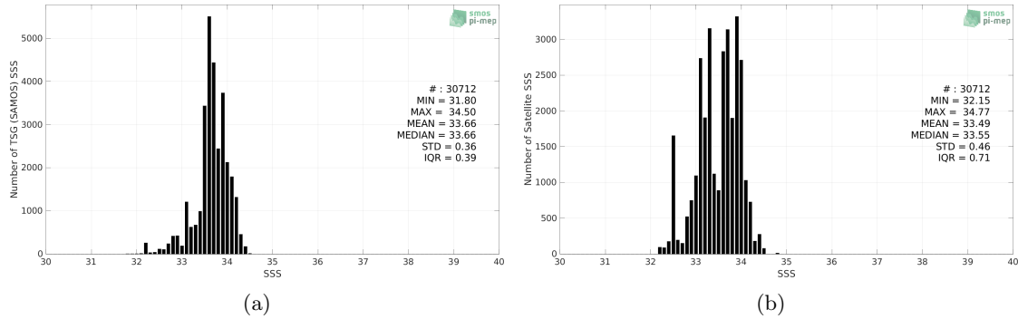
Figure 2: Histograms of SSS from TSG (SAMOS) (a) and SMAP SSS L3 v5 - 8-Day running (RSS) (b) considering all match-up pairs per bins of 0.1 over the South China Sea Pi-MEP region and for the full satellite product period.
