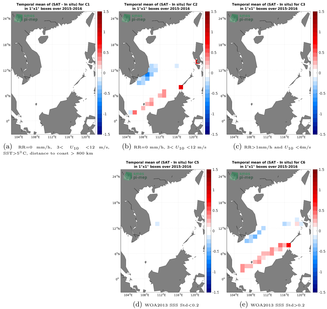
Figure 12: Temporal mean gridded over spatial boxes of size 1^\circ \times 1^\circ of \Delta SSS (SMAP SSS L3 v5 - 8-Day running (RSS) - TSG (SAMOS)) for 5 different subdatasets corresponding to: RR=0 mm/h, 3 < U_{10} < 12 m/s, SST > 5°C, distance to coast > 800 km (a), RR=0 mm/h, 3 < U_{10} < 12 m/s (b), RR > 1mm/h and U_{10} < 4 m/s (c), WOA2013 SSS Std < 0.2 (d), WOA2013 SSS Std > 0.2 (e).
