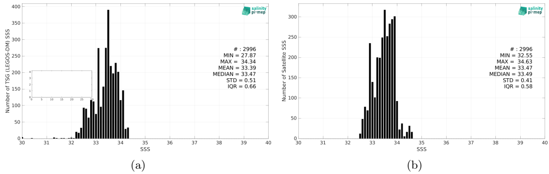
Figure 2: Histograms of SSS from TSG (LEGOS-DM) (a) and SMAP SSS L3 v5 - 8-Day running (RSS) (b) considering all match-up pairs per bins of 0.1 over the South China Sea Pi-MEP region and for the full satellite product period.
