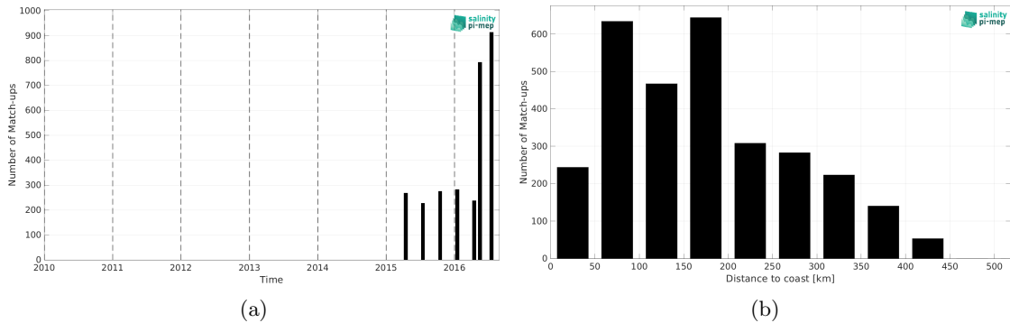
Figure 1: Number of match-ups between TSG (LEGOS-DM) and SMAP SSS L3 v5 - 8-Day running (RSS) SSS as a function of time (a) and as function of the distance to coast (b) over the South China Sea Pi-MEP region and for the full satellite product period.
