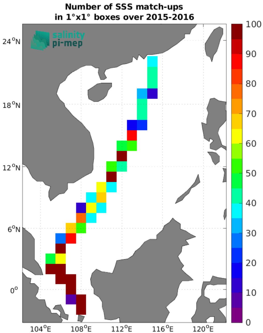
Figure 4: Number of SSS match-ups between TSG (LEGOS-DM) SSS and the SMAP SSS L3 v5 - 8-Day running (RSS) SSS product for the South China Sea Pi-MEP region over 1°x1° boxes and for the full satellite product period.
