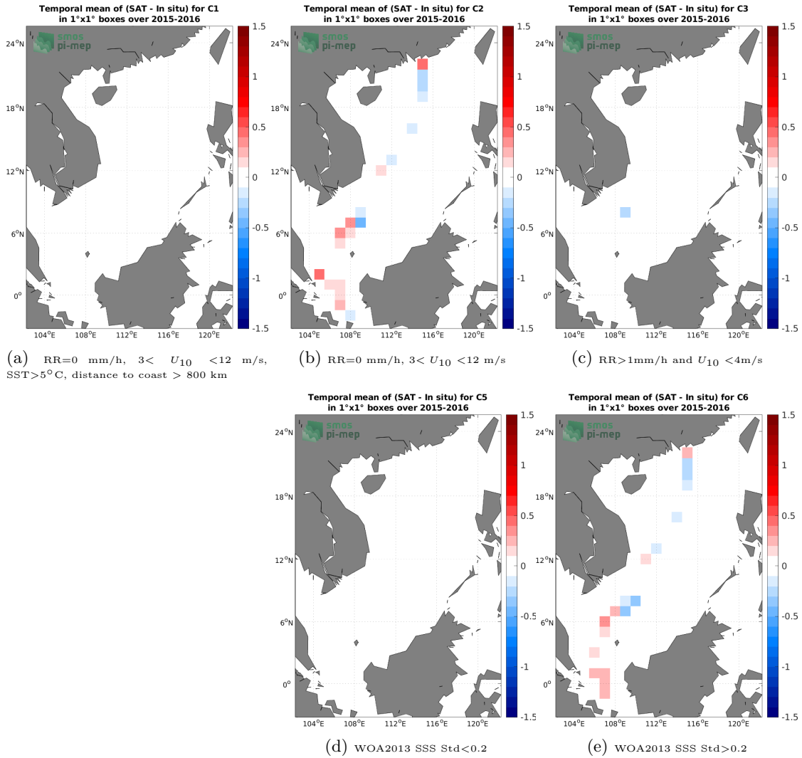
Figure 12: Temporal mean gridded over spatial boxes of size 1^\circ \times 1^\circ of \Delta SSS (SMAP SSS L3 v5 - 8-Day running (RSS) - TSG (LEGOS-DM)) for 5 different subdatasets corresponding to: RR=0 mm/h, 3 < U_{10} < 12 m/s, SST > 5°C, distance to coast > 800 km (a), RR=0 mm/h, 3 < U_{10} < 12 m/s (b), RR > 1mm/h and U_{10} < 4 m/s (c), WOA2013 SSS Std < 0.2 (d), WOA2013 SSS Std > 0.2 (e).
