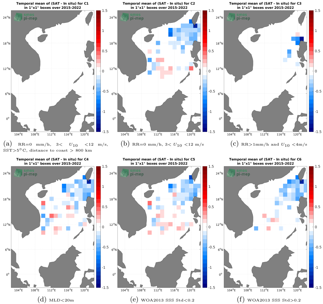
Figure 12: Temporal mean gridded over spatial boxes of size 1^\circ \times 1^\circ of \Delta\text{SSS} (SMAP SSS L3 v5 - 8-Day running (RSS) - Argo) for 6 different subdatasets corresponding to: RR=0 mm/h, 3 < U_{10} < 12 m/s, SST > 5^\circ\text{C} , distance to coast > 800 km (a), RR=0 mm/h, 3 < U_{10} < 12 m/s (b), RR > 1\text{mm/h} and U_{10} < 4\text{m/s} (c), MLD < 20\text{m} (d), WOA2013 SSS Std < 0.2 (e), WOA2013 SSS Std > 0.2 (f).
