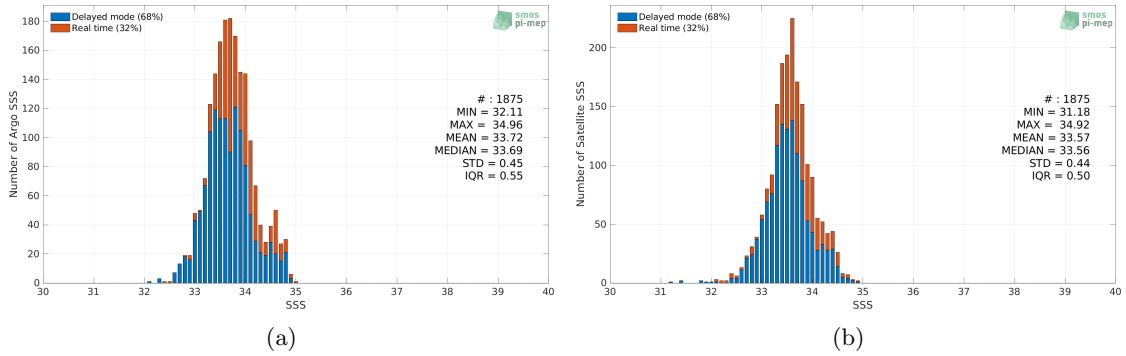
Figure 2: Histograms of SSS from Argo (a) and SMAP SSS L3 v5 - 8-Day running (RSS) (b) considering all match-up pairs per bins of 0.1 over the South China Sea Pi-MEP region and for the full satellite product period.
