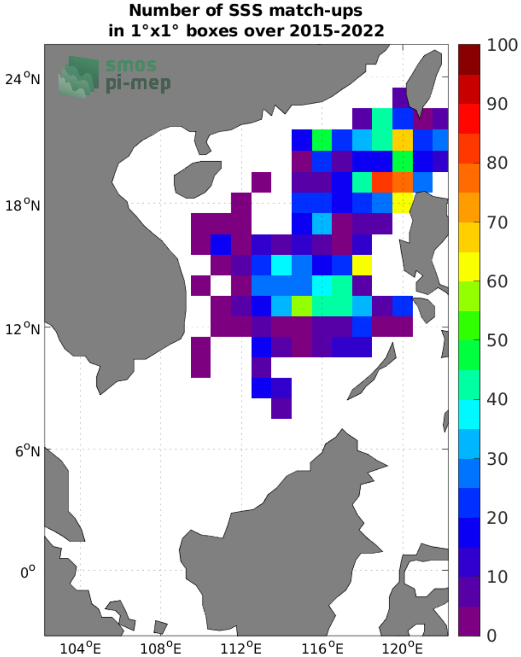
Figure 4: Number of SSS match-ups between Argo SSS and the SMAP SSS L3 v5 - 8-Day running (RSS) SSS product for the South China Sea Pi-MEP region over 1^\circ \times 1^\circ boxes and for the full satellite product period.
