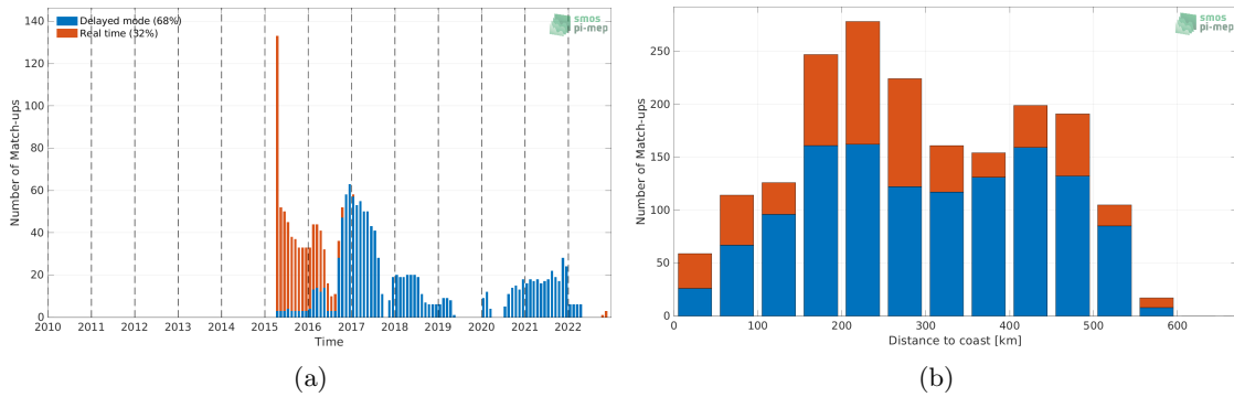
Figure 1: Number of match-ups between Argo and SMAP SSS L3 v5 - 8-Day running (RSS) SSS as a function of time (a) and as function of the distance to coast (b) over the South China Sea Pi-MEP region and for the full satellite product period.
