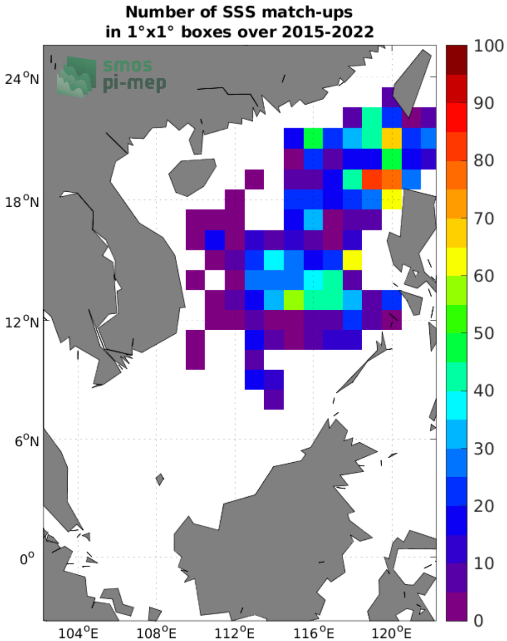
Figure 4: Number of SSS match-ups between Argo SSS and the SMAP SSS L3 v5 - 8-Day running (RSS) SSS product for the South China Sea Pi-MEP region over 1°x1° boxes and for the full satellite product period.
