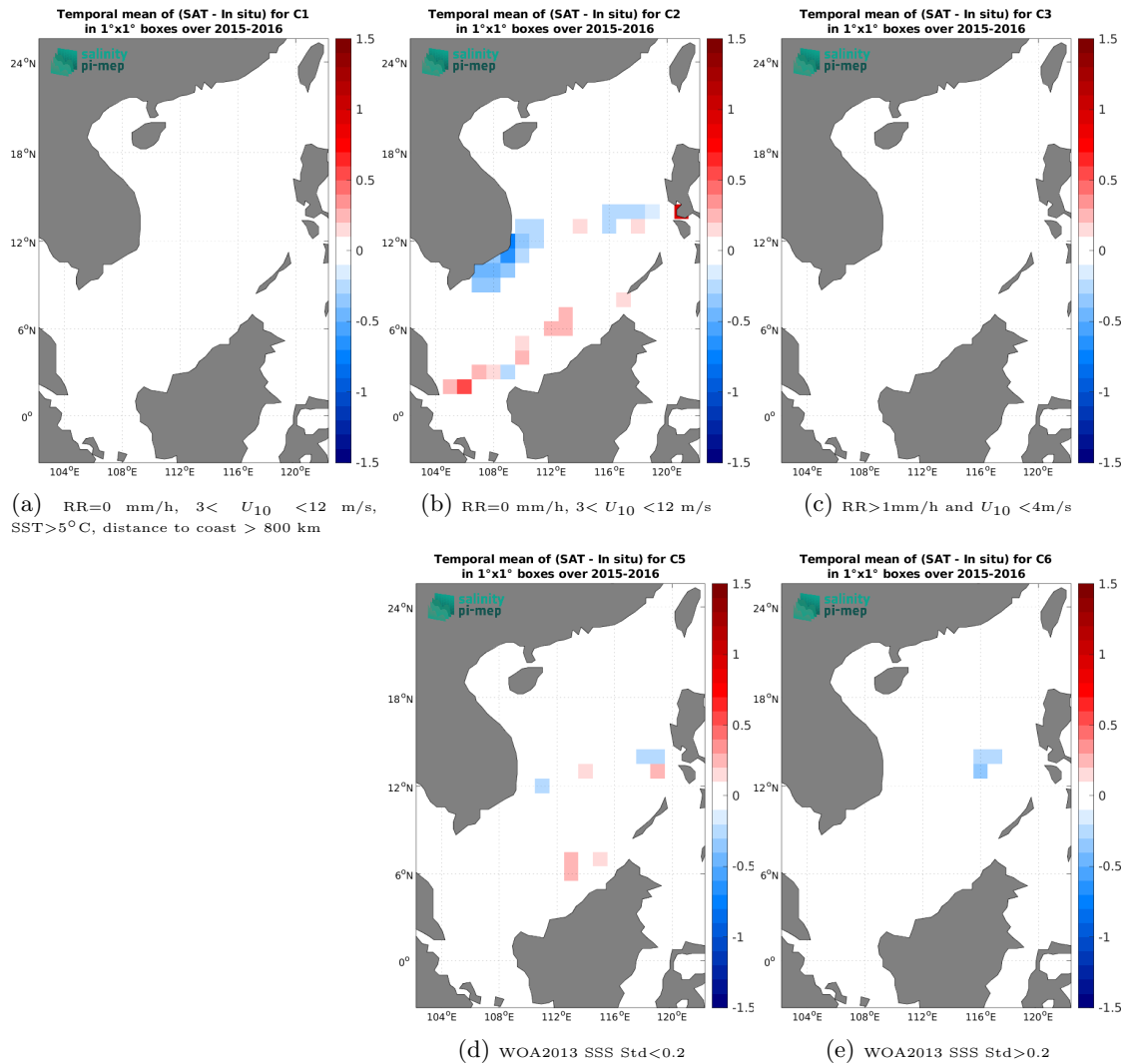
Figure 12: Temporal mean gridded over spatial boxes of size 1^\circ \times 1^\circ of \Delta\text{SSS} (SMAP SSS L3 v5 - Monthly (RSS) - TSG (SAMOS)) for 5 different subdatasets corresponding to:RR=0 mm/h, 3 < U_{10} < 12 m/s, SST >5^\circ\text{C} , distance to coast > 800 km (a), RR=0 mm/h, 3 < U_{10} < 12 m/s (b), RR >1 mm/h and U_{10} < 4 m/s (c), WOA2013 SSS Std <0.2 (d), WOA2013 SSS Std >0.2 (e).
