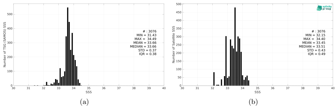
Figure 2: Histograms of SSS from TSG (SAMOS) (a) and SMAP SSS L3 v5 - Monthly (RSS) (b) considering all match-up pairs per bins of 0.1 over the South China Sea Pi-MEP region and for the full satellite product period.
