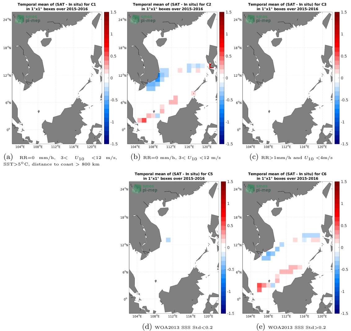
Figure 12: Temporal mean gridded over spatial boxes of size 1^\circ \times 1^\circ of \Delta SSS (SMAP SSS L3 v5 - Monthly (RSS) - TSG (SAMOS)) for 5 different subdatasets corresponding to:RR=0 mm/h, 3 < U_{10} < 12 m/s, SST>5°C, distance to coast > 800 km (a), RR=0 mm/h, 3 < U_{10} < 12 m/s (b), RR>1mm/h and U_{10} < 4 m/s (c), WOA2013 SSS Std<0.2 (d), WOA2013 SSS Std>0.2 (e).
