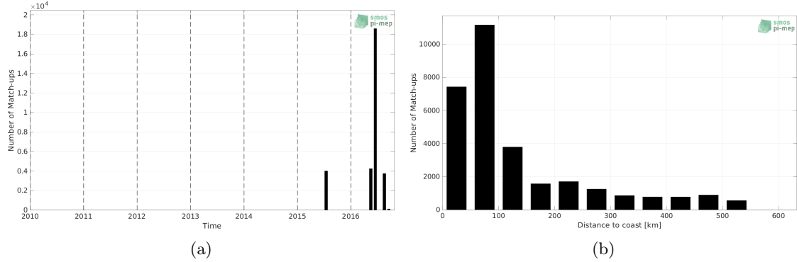
Figure 1: Number of match-ups between TSG (SAMOS) and SMAP SSS L3 v5 - Monthly (RSS) SSS as a function of time (a) and as function of the distance to coast (b) over the South China Sea Pi-MEP region and for the full satellite product period.
