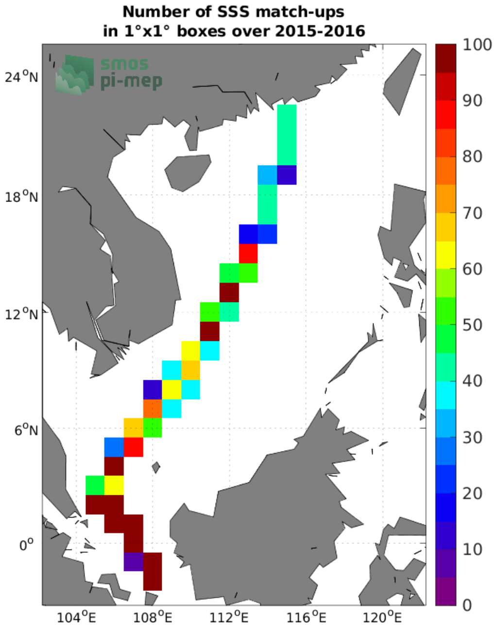
Figure 4: Number of SSS match-ups between TSG (LEGOS-DM) SSS and the SMAP SSS L3 v5 - Monthly (RSS) SSS product for the South China Sea Pi-MEP region over 1°×1° boxes and for the full satellite product period.
