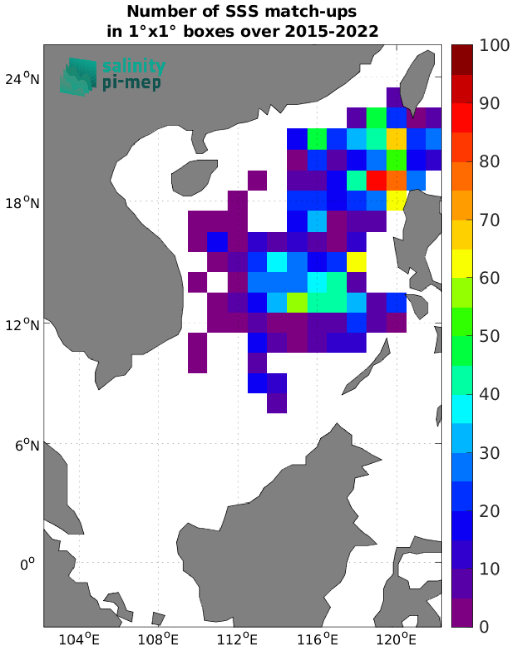
Figure 4: Number of SSS match-ups between Argo SSS and the SMAP SSS L3 v5 - Monthly (RSS) SSS product for the South China Sea Pi-MEP region over 1^\circ \times 1^\circ boxes and for the full satellite product period.
