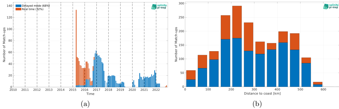
Figure 1: Number of match-ups between Argo and SMAP SSS L3 v5 - Monthly (RSS) SSS as a function of time (a) and as function of the distance to coast (b) over the South China Sea Pi-MEP region and for the full satellite product period.
