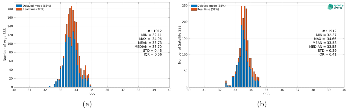
Figure 2: Histograms of SSS from Argo (a) and SMAP SSS L3 v5 - Monthly (RSS) (b) considering all match-up pairs per bins of 0.1 over the South China Sea Pi-MEP region and for the full satellite product period.
