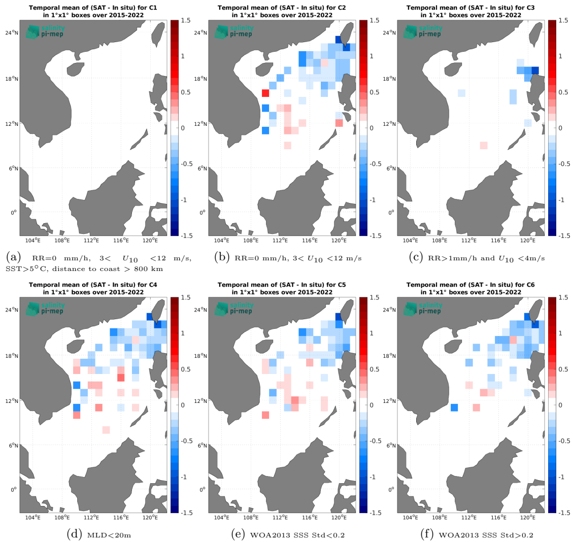
Figure 12: Temporal mean gridded over spatial boxes of size 1^\circ \times 1^\circ of \Delta\text{SSS} (SMAP SSS L3 v5 - Monthly (RSS) - Argo) for 6 different subdatasets corresponding to: RR=0 mm/h, 3 < U_{10} < 12 m/s, SST > 5^\circ\text{C} , distance to coast > 800 km (a), RR=0 mm/h, 3 < U_{10} < 12 m/s (b), RR > 1 mm/h and U_{10} < 4 m/s (c), MLD < 20 m (d), WOA2013 SSS Std < 0.2 (e), WOA2013 SSS Std > 0.2 (f).
