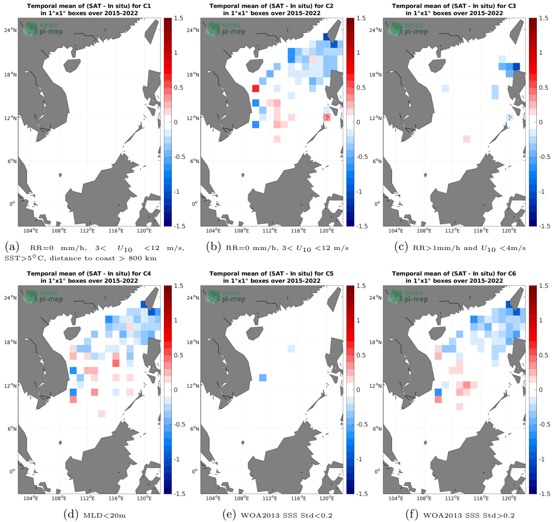
Figure 12: Temporal mean gridded over spatial boxes of size 1^\circ \times 1^\circ of \Delta SSS (SMAP SSS L3 v5 - Monthly (RSS) - Argo) for 6 different subdatasets corresponding to:RR=0 mm/h, 3 < U_{10} < 12 m/s, SST>5°C, distance to coast > 800 km (a), RR=0 mm/h, 3 < U_{10} < 12 m/s (b), RR>1mm/h and U_{10} < 4 m/s (c),MLD<20m (d),WOA2013 SSS Std<0.2 (e),WOA2013 SSS Std>0.2 (f).
