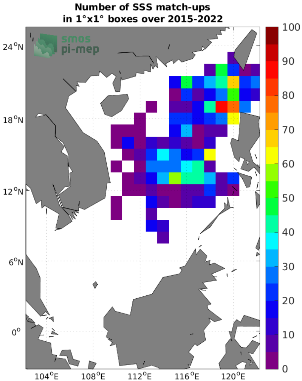
Figure 4: Number of SSS match-ups between Argo SSS and the SMAP SSS L3 v5 - Monthly (RSS) SSS product for the South China Sea Pi-MEP region over 1°x1° boxes and for the full satellite product period.
