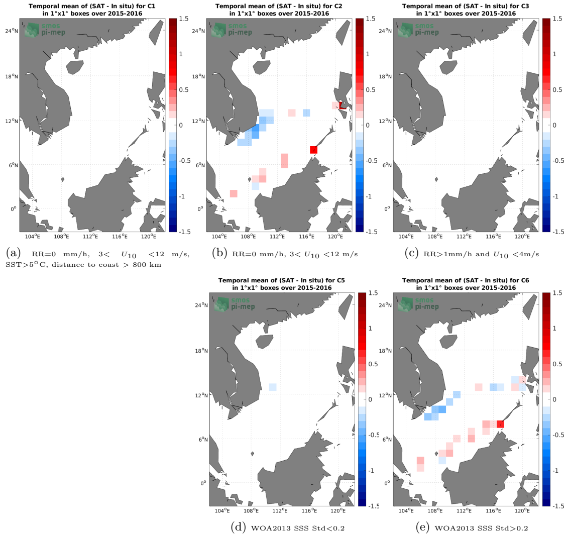
Figure 12: Temporal mean gridded over spatial boxes of size 1^\circ \times 1^\circ of \Delta SSS (SMAP SSS L3 v4 - 8-Day running (RSS) - TSG (SAMOS)) for 5 different subdatasets corresponding to: RR=0 mm/h, 3 < U_{10} < 12 m/s, SST > 5°C, distance to coast > 800 km (a), RR=0 mm/h, 3 < U_{10} < 12 m/s (b), RR > 1mm/h and U_{10} < 4 m/s (c), WOA2013 SSS Std < 0.2 (d), WOA2013 SSS Std > 0.2 (e).
