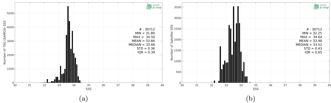
Figure 2: Histograms of SSS from TSG (SAMOS) (a) and SMAP SSS L3 v4 - 8-Day running (RSS) (b) considering all match-up pairs per bins of 0.1 over the South China Sea Pi-MEP region and for the full satellite product period.
