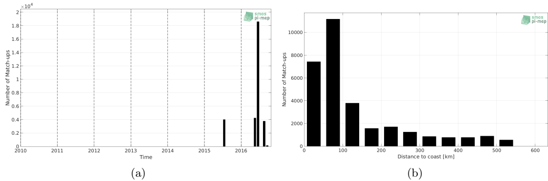
Figure 1: Number of match-ups between TSG (SAMOS) and SMAP SSS L3 v4 - 8-Day running (RSS) SSS as a function of time (a) and as function of the distance to coast (b) over the South China Sea Pi-MEP region and for the full satellite product period.
