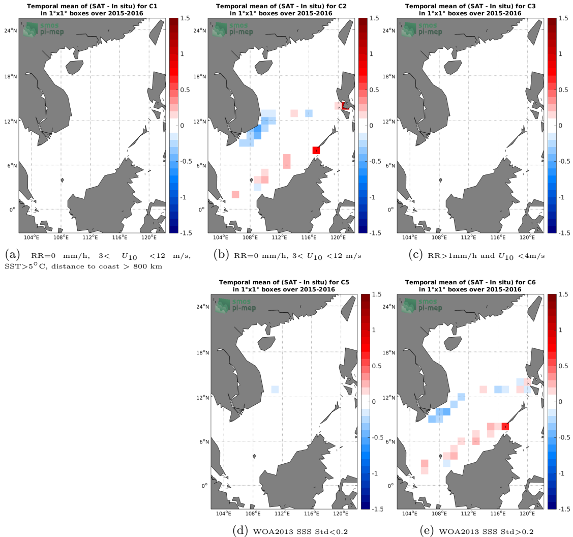
Figure 12: Temporal mean gridded over spatial boxes of size 1^\circ \times 1^\circ of \Delta\text{SSS} (SMAP SSS L3 v4 - 8-Day running (RSS) - TSG (SAMOS)) for 5 different subdatasets corresponding to: RR=0 mm/h, 3 < U_{10} < 12 m/s, SST > 5^\circ\text{C} , distance to coast > 800 km (a), RR=0 mm/h, 3 < U_{10} < 12 m/s (b), RR > 1 mm/h and U_{10} < 4 m/s (c), WOA2013 SSS Std < 0.2 (d), WOA2013 SSS Std > 0.2 (e).
