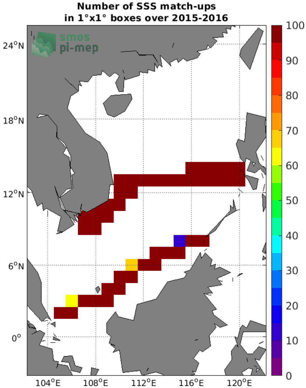
Figure 4: Number of SSS match-ups between TSG (SAMOS) SSS and the SMAP SSS L3 v4 - 8-Day running (RSS) SSS product for the South China Sea Pi-MEP region over 1°x1° boxes and for the full satellite product period.
