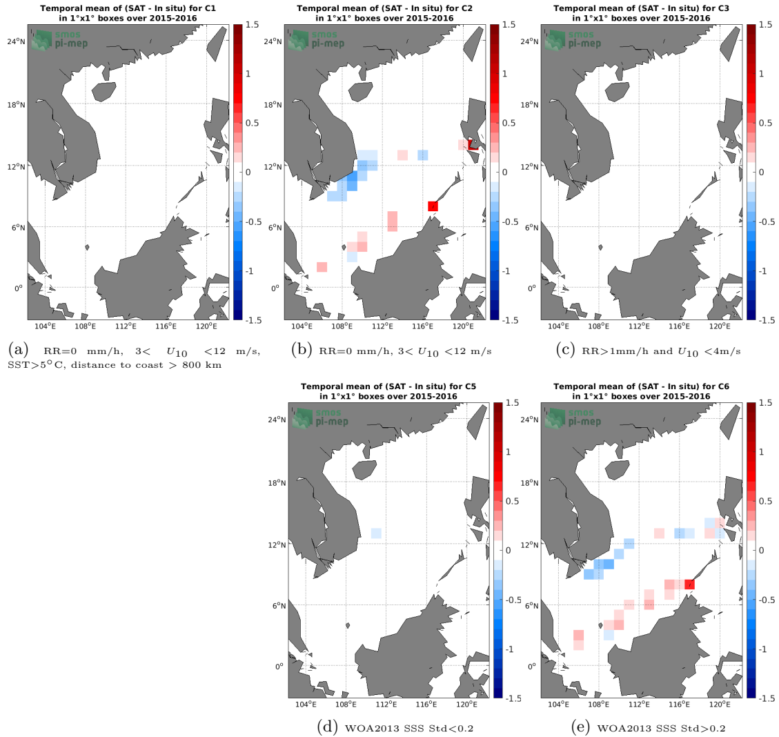
Figure 12: Temporal mean gridded over spatial boxes of size 1°x1° of \Delta SSS (SMAP SSS L3 v4 - 8-Day running (RSS) - TSG (SAMOS)) for 5 different subdatasets corresponding to:RR=0 mm/h, 3 < U_{10} < 12 m/s, SST>5°C, distance to coast > 800 km (a), RR=0 mm/h, 3 < U_{10} < 12 m/s (b), RR>1mm/h and U_{10} < 4 m/s (c), WOA2013 SSS Std<0.2 (d), WOA2013 SSS Std>0.2 (e).
