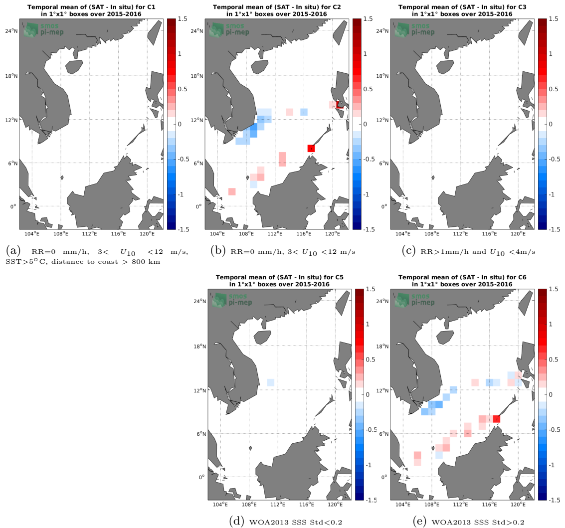
Figure 12: Temporal mean gridded over spatial boxes of size 1^\circ \times 1^\circ of \Delta SSS (SMAP-L3-RSS-V4-8DAY-RUNNING - TSG-SAMOS) for 5 different subdatasets corresponding to:RR=0 mm/h, 3 < U_{10} < 12 m/s, SST >5^\circ C, distance to coast > 800 km (a), RR=0 mm/h, 3 < U_{10} < 12 m/s (b), RR >1 mm/h and U_{10} < 4 m/s (c), WOA2013 SSS Std <0.2 (d), WOA2013 SSS Std >0.2 (e).
