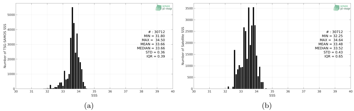
Figure 2: Histograms of SSS from TSG-SAMOS (a) and SMAP-L3-RSS-V4-8DAY-RUNNING (b) considering all match-up pairs per bins of 0.1 over the South China Sea Pi-MEP region and for the full satellite product period.
