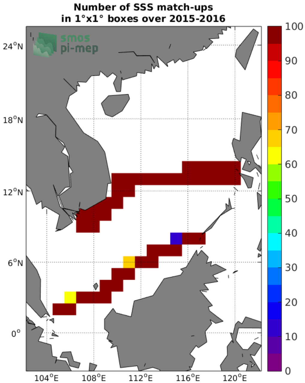
Figure 4: Number of SSS match-ups between TSG-SAMOS SSS and the SMAP-L3-RSS-V4-8DAY-RUNNING SSS product for the South China Sea Pi-MEP region over 1°x1° boxes and for the full satellite product period.
