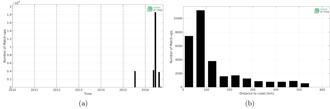
Figure 1: Number of match-ups between TSG-SAMOS and SMAP-L3-RSS-V4-8DAY-RUNNING SSS as a function of time (a) and as function of the distance to coast (b) over the South China Sea Pi-MEP region and for the full satellite product period.
