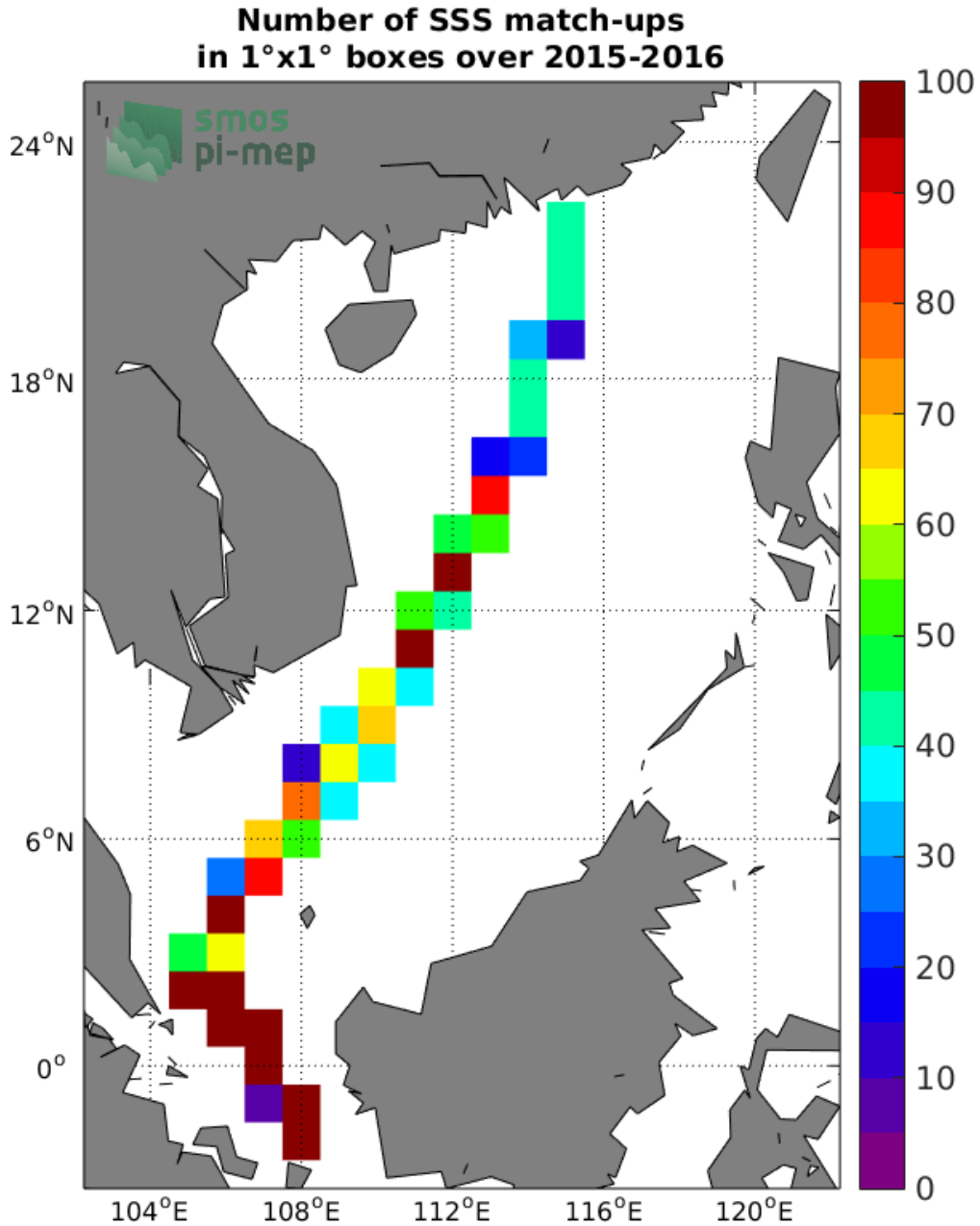
Figure 4: Number of SSS match-ups between TSG (LEGOS-DM) SSS and the SMAP SSS L3 v4 - 8-Day running (RSS) SSS product for the South China Sea Pi-MEP region over 1°x1° boxes and for the full satellite product period.
