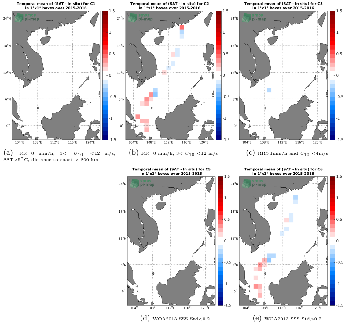
Figure 12: Temporal mean gridded over spatial boxes of size 1^\circ \times 1^\circ of \Delta\text{SSS} (SMAP SSS L3 v4 - 8-Day running (RSS) - TSG (LEGOS-DM)) for 5 different subdatasets corresponding to: RR=0 mm/h, 3 < U_{10} < 12 m/s, SST > 5^\circ\text{C} , distance to coast > 800 km (a), RR=0 mm/h, 3 < U_{10} < 12 m/s (b), RR > 1 mm/h and U_{10} < 4 m/s (c), WOA2013 SSS Std < 0.2 (d), WOA2013 SSS Std > 0.2 (e).
