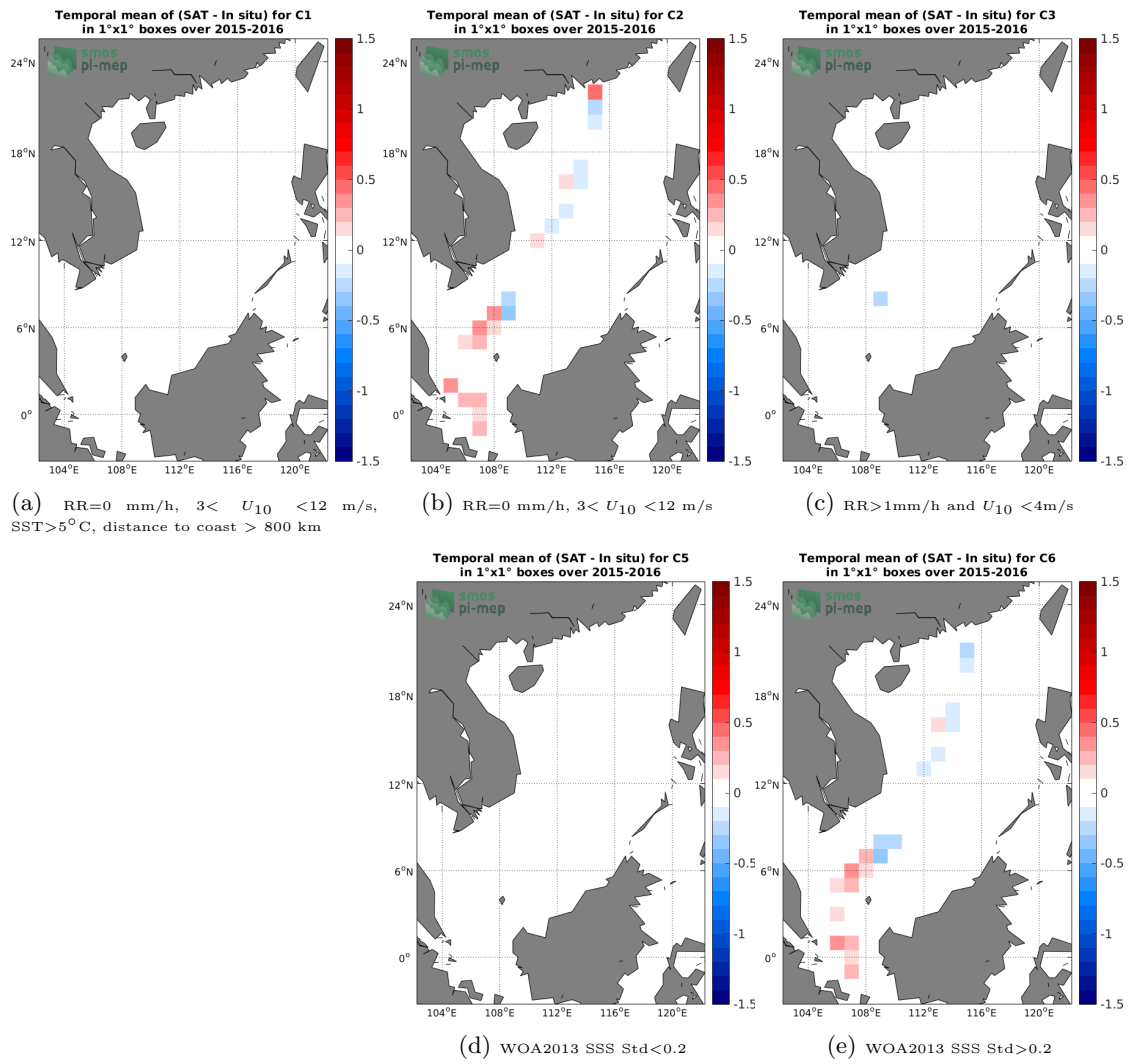
Figure 12: Temporal mean gridded over spatial boxes of size 1°x1° of \Delta SSS (SMAP-L3-RSS-V4-8DAY-RUNNING - TSG-LEGOS-DM) for 5 different subdatasets corresponding to: RR=0 mm/h, 3 < U_{10} < 12 m/s, SST > 5°C, distance to coast > 800 km (a), RR=0 mm/h, 3 < U_{10} < 12 m/s (b), RR > 1mm/h and U_{10} < 4 m/s (c), WOA2013 SSS Std < 0.2 (d), WOA2013 SSS Std > 0.2 (e).
