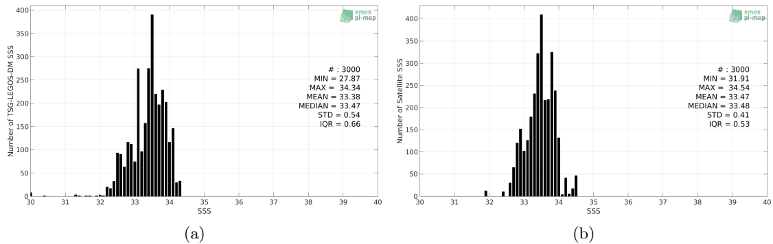
Figure 2: Histograms of SSS from TSG-LEGOS-DM (a) and SMAP-L3-RSS-V4-8DAY-RUNNING (b) considering all match-up pairs per bins of 0.1 over the South China Sea Pi-MEP region and for the full satellite product period.
