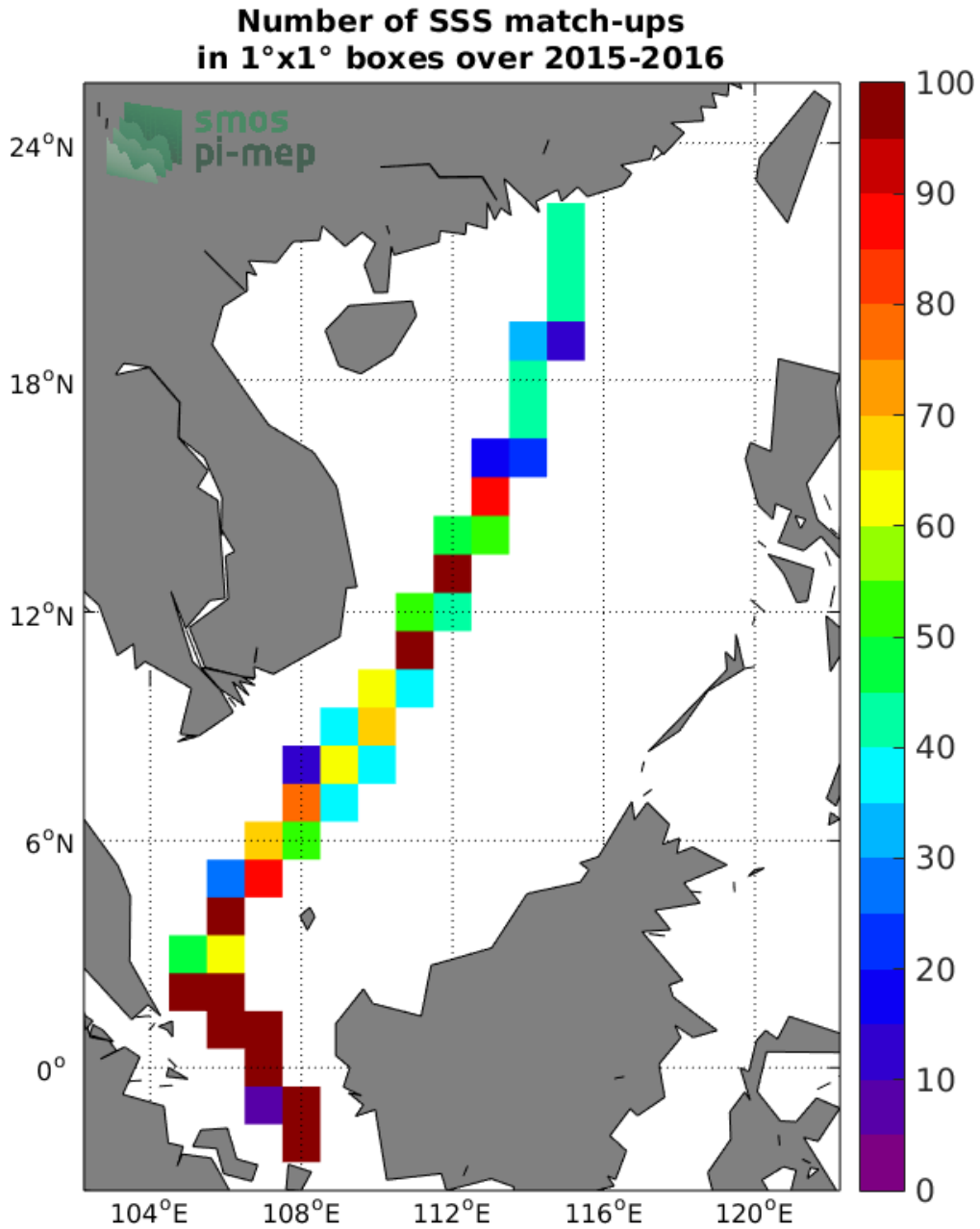
Figure 4: Number of SSS match-ups between TSG-LEGOS-DM SSS and the SMAP-L3-RSS-V4-8DAY-RUNNING SSS product for the South China Sea Pi-MEP region over 1°x1° boxes and for the full satellite product period.
