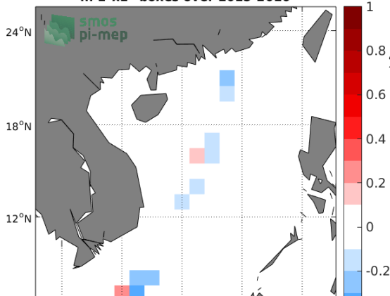
Temporal mean of (Sat - TSG-LEGOS-DM) in 1°x1° boxes over 2015-2016
