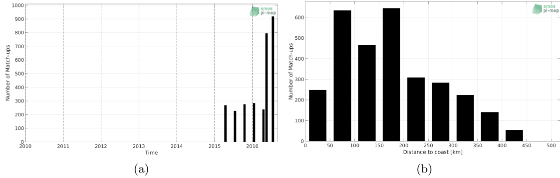
Figure 1: Number of match-ups between TSG-LEGOS-DM and SMAP-L3-RSS-V4-8DAY-RUNNING SSS as a function of time (a) and as function of the distance to coast (b) over the South China Sea Pi-MEP region and for the full satellite product period.
