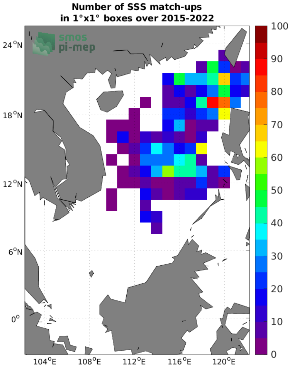
Figure 4: Number of SSS match-ups between Argo SSS and the SMAP SSS L3 v4 - 8-Day running (RSS) SSS product for the South China Sea Pi-MEP region over 1^\circ \times 1^\circ boxes and for the full satellite product period.
