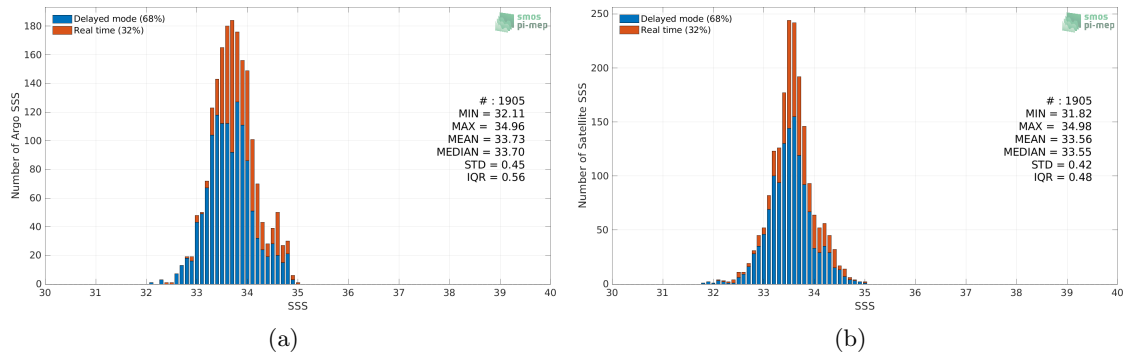
Figure 2: Histograms of SSS from Argo (a) and SMAP SSS L3 v4 - 8-Day running (RSS) (b) considering all match-up pairs per bins of 0.1 over the South China Sea Pi-MEP region and for the full satellite product period.
