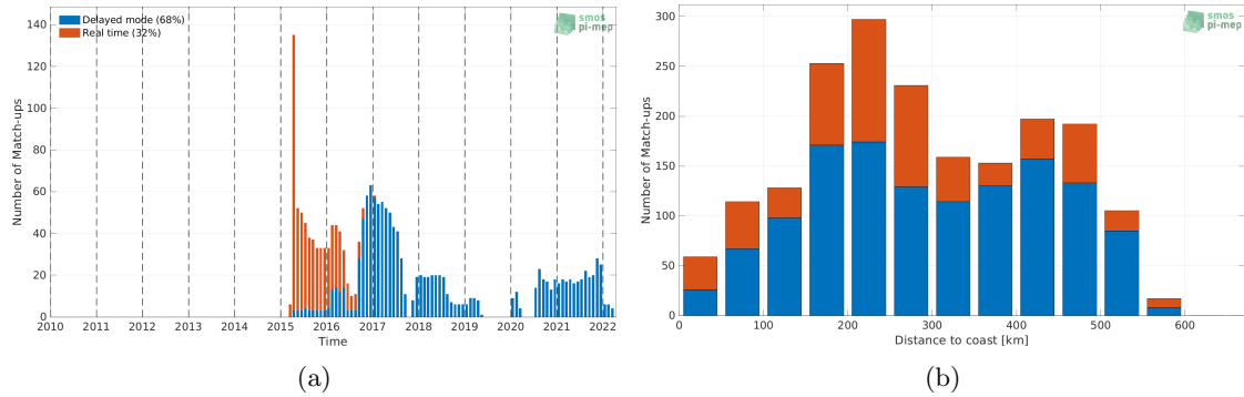
Figure 1: Number of match-ups between Argo and SMAP SSS L3 v4 - 8-Day running (RSS) SSS as a function of time (a) and as function of the distance to coast (b) over the South China Sea Pi-MEP region and for the full satellite product period.
