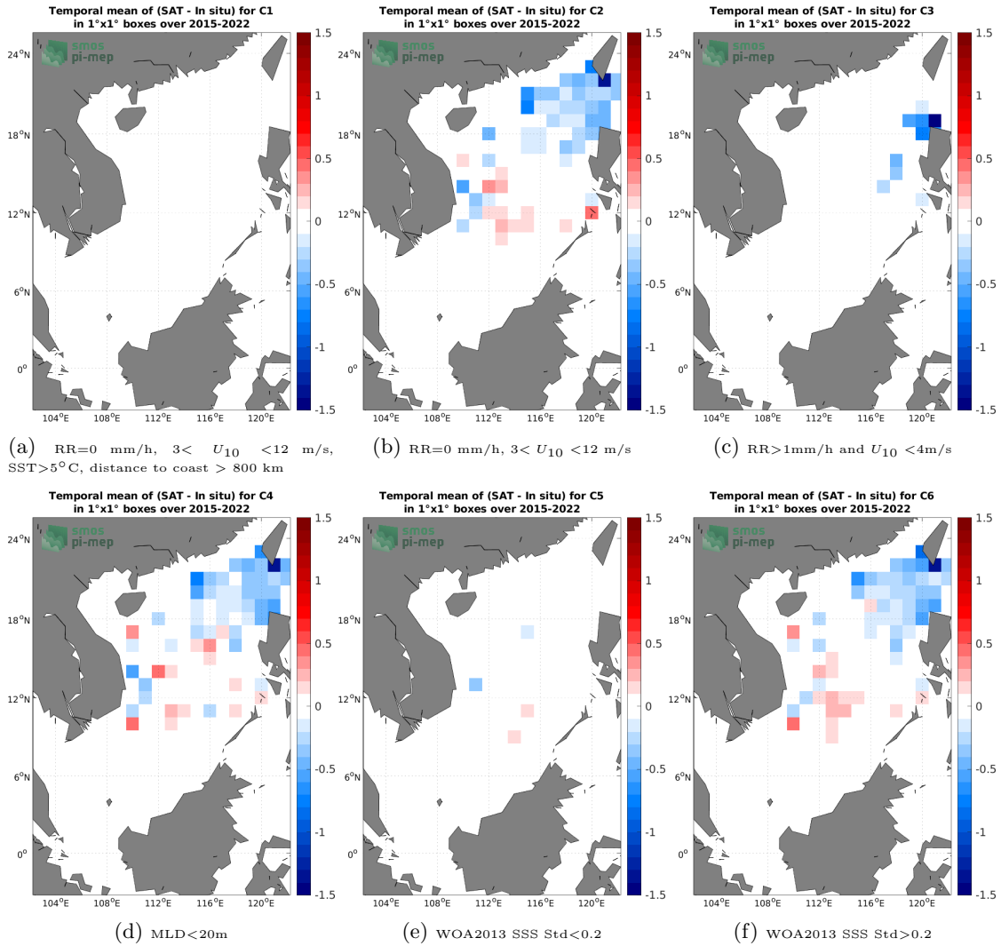
Figure 12: Temporal mean gridded over spatial boxes of size 1^\circ \times 1^\circ of \Delta\text{SSS} (SMAP SSS L3 v4 - 8-Day running (RSS) - Argo) for 6 different subdatasets corresponding to: RR=0 mm/h, 3 < U_{10} < 12 m/s, SST > 5^\circ\text{C} , distance to coast > 800 km (a), RR=0 mm/h, 3 < U_{10} < 12 m/s (b), RR > 1 mm/h and U_{10} < 4 m/s (c), MLD < 20 m (d), WOA2013 SSS Std < 0.2 (e), WOA2013 SSS Std > 0.2 (f).
