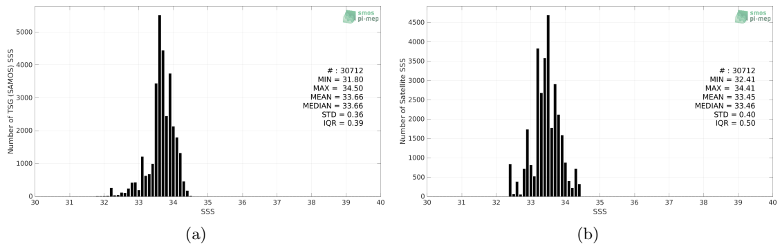
Figure 2: Histograms of SSS from TSG (SAMOS) (a) and SMAP SSS L3 v4 - Monthly (RSS) (b) considering all match-up pairs per bins of 0.1 over the South China Sea Pi-MEP region and for the full satellite product period.
