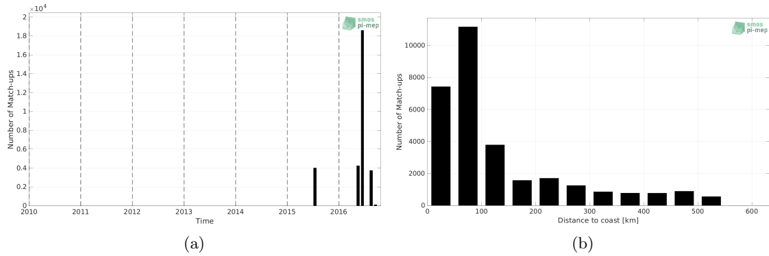
Figure 1: Number of match-ups between TSG (SAMOS) and SMAP SSS L3 v4 - Monthly (RSS) SSS as a function of time (a) and as function of the distance to coast (b) over the South China Sea Pi-MEP region and for the full satellite product period.
