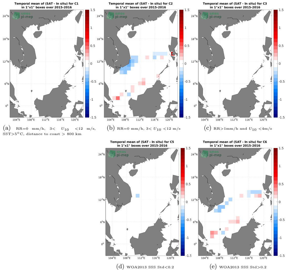
Figure 12: Temporal mean gridded over spatial boxes of size 1^\circ \times 1^\circ of \Delta SSS (SMAP SSS L3 v4 - Monthly (RSS) - TSG (SAMOS)) for 5 different subdatasets corresponding to:RR=0 mm/h, 3 < U_{10} < 12 m/s, SST>5°C, distance to coast > 800 km (a), RR=0 mm/h, 3 < U_{10} < 12 m/s (b), RR>1mm/h and U_{10} < 4 m/s (c), WOA2013 SSS Std<0.2 (d), WOA2013 SSS Std>0.2 (e).
