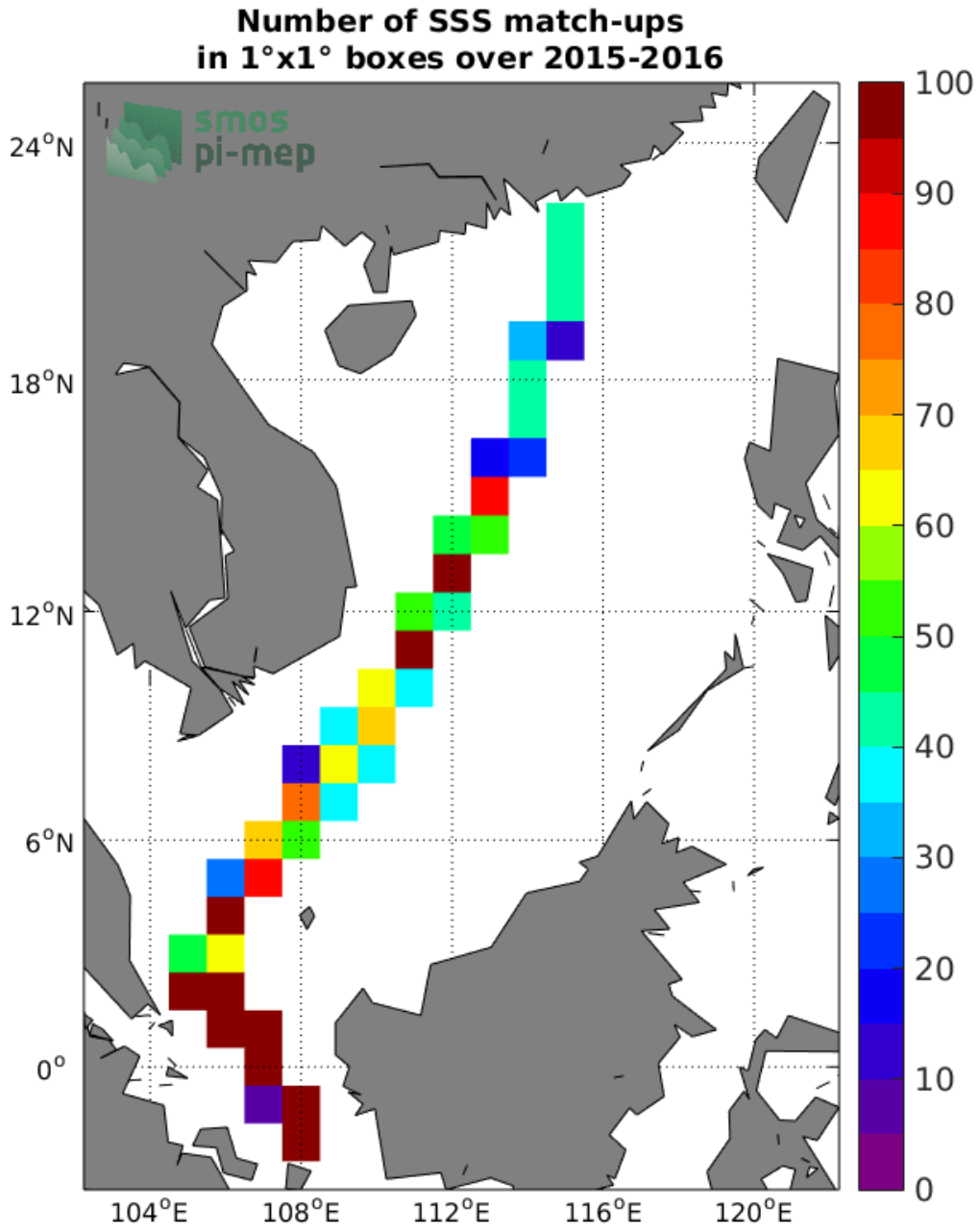
Figure 4: Number of SSS match-ups between TSG-LEGOS-DM SSS and the SMAP-L3-RSS-V4-MONTHLY SSS product for the South China Sea Pi-MEP region over 1°x1° boxes and for the full satellite product period.
