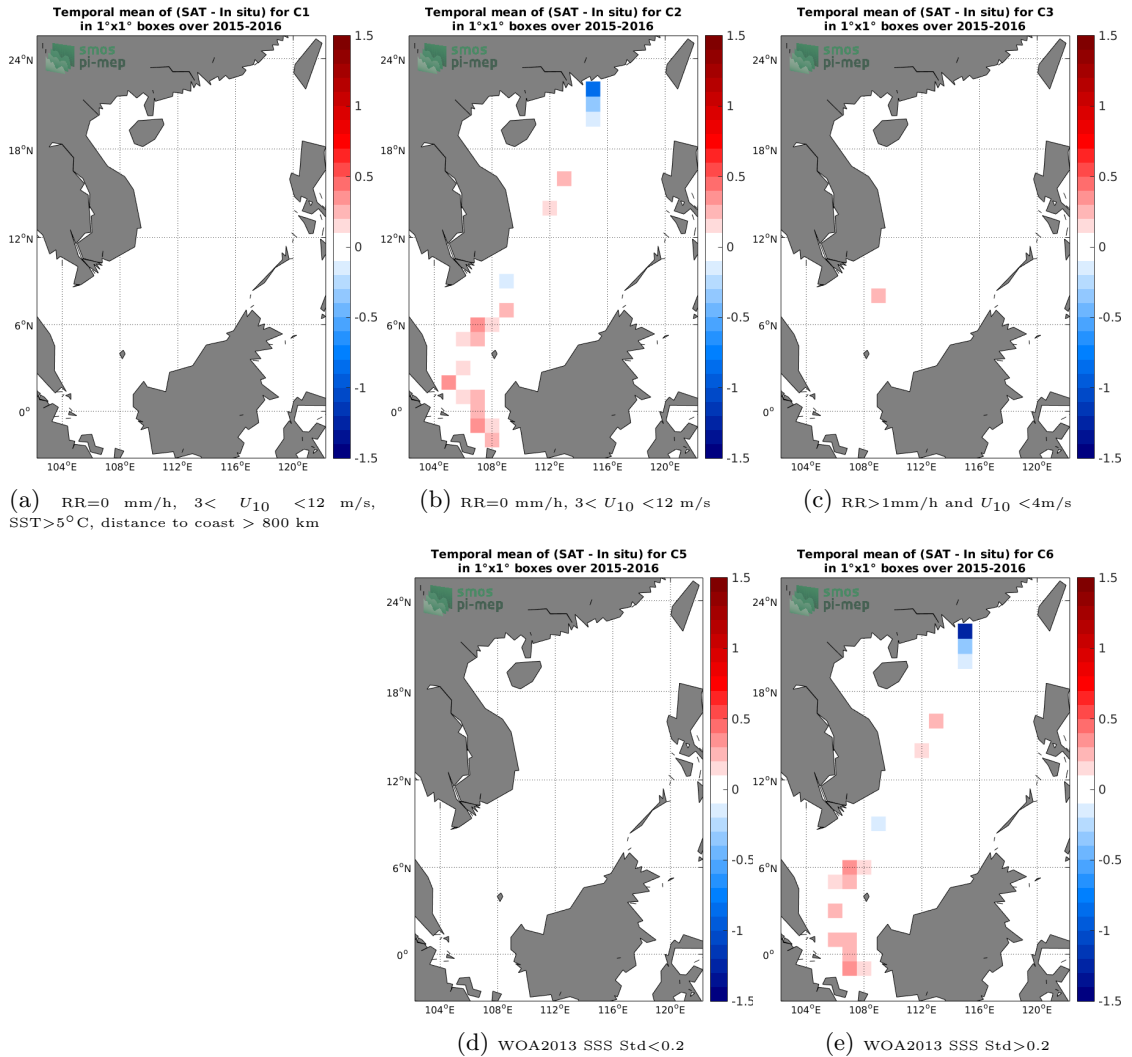
Figure 12: Temporal mean gridded over spatial boxes of size 1°x1° of \Delta SSS (SMAP-L3-RSS-V4-MONTHLY - TSG-LEGOS-DM) for 5 different subdatasets corresponding to:RR=0 mm/h, 3 < U_{10} < 12 m/s, SST>5°C, distance to coast > 800 km (a), RR=0 mm/h, 3 < U_{10} < 12 m/s (b), RR>1mm/h and U_{10} < 4 m/s (c), WOA2013 SSS Std<0.2 (d), WOA2013 SSS Std>0.2 (e).
