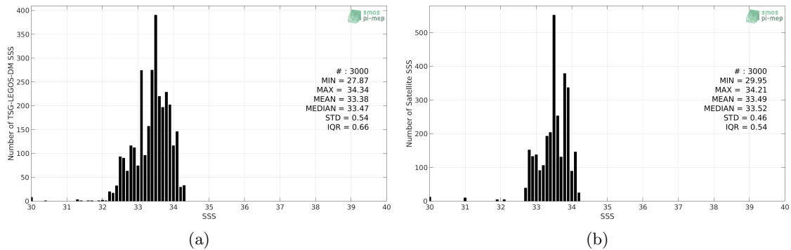
Figure 2: Histograms of SSS from TSG-LEGOS-DM (a) and SMAP-L3-RSS-V4-MONTHLY (b) considering all match-up pairs per bins of 0.1 over the South China Sea Pi-MEP region and for the full satellite product period.
