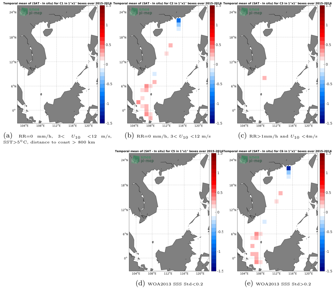
Figure 12: Temporal mean gridded over spatial boxes of size 1^\circ \times 1^\circ of \Delta SSS (SMAP-L3-RSS-V4-MONTHLY - TSG-LEGOS-DM) for 5 different subdatasets corresponding to:RR=0 mm/h, 3 < U_{10} < 12 m/s, SST>5°C, distance to coast > 800 km (a), RR=0 mm/h, 3 < U_{10} < 12 m/s (b), RR>1mm/h and U_{10} < 4 m/s (c), WOA2013 SSS Std<0.2 (d), WOA2013 SSS Std>0.2 (e).
