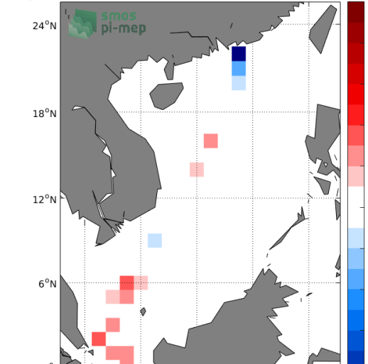
Temporal mean of (Sat - TSG-LEGOS-DM) in 1°x1° boxes over 2015-2016
