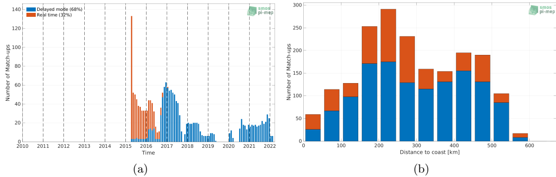
Figure 1: Number of match-ups between Argo and SMAP SSS L3 v4 - Monthly (RSS) SSS as a function of time (a) and as function of the distance to coast (b) over the South China Sea Pi-MEP region and for the full satellite product period.
