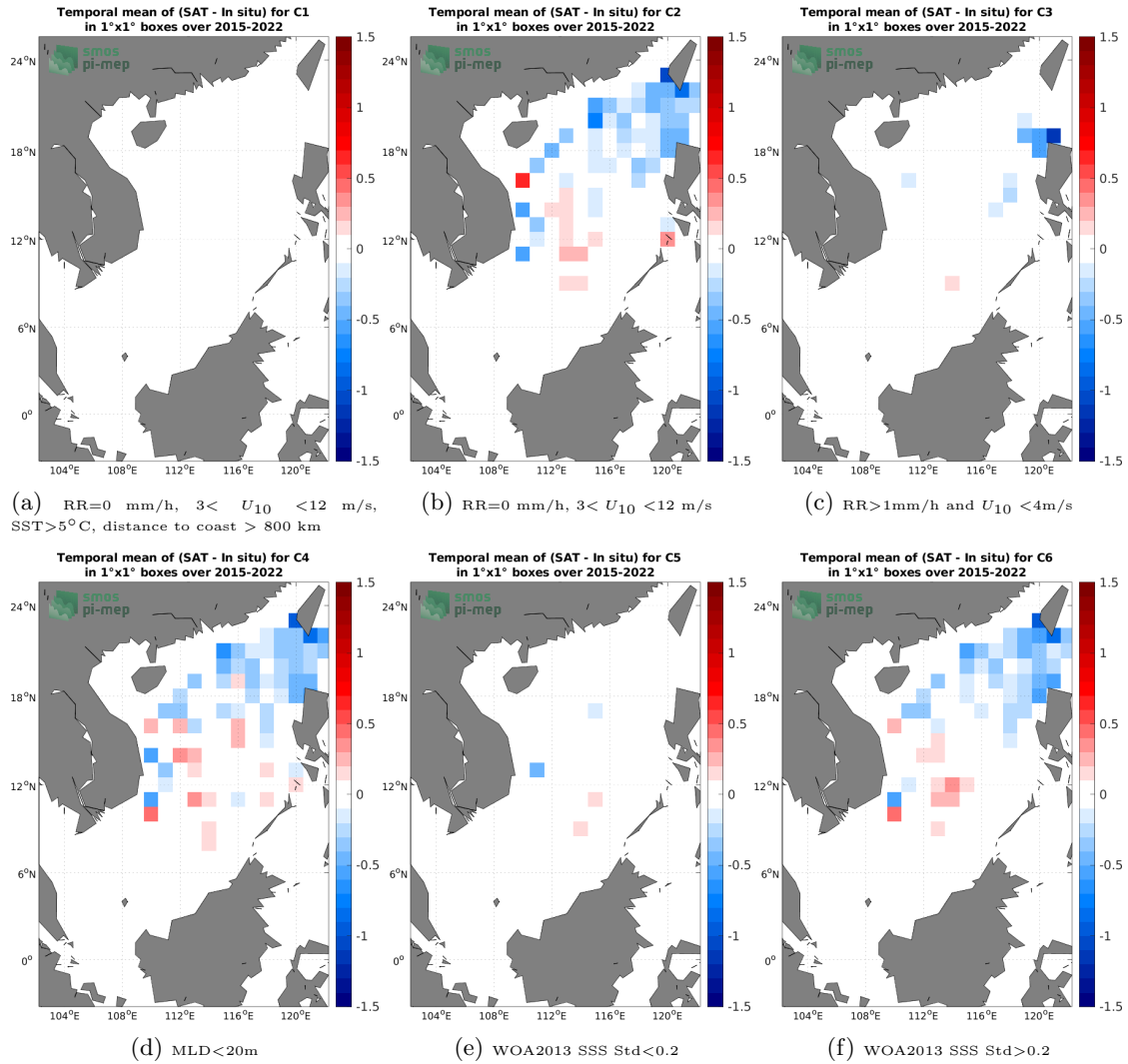
Figure 12: Temporal mean gridded over spatial boxes of size 1^\circ \times 1^\circ of \Delta\text{SSS} (SMAP SSS L3 v4 - Monthly (RSS) - Argo) for 6 different subdatasets corresponding to: RR=0 mm/h, 3 < U_{10} < 12 m/s, SST > 5^\circ\text{C} , distance to coast > 800 km (a), RR=0 mm/h, 3 < U_{10} < 12 m/s (b), RR > 1 mm/h and U_{10} < 4 m/s (c), MLD < 20 m (d), WOA2013 SSS Std < 0.2 (e), WOA2013 SSS Std > 0.2 (f).
