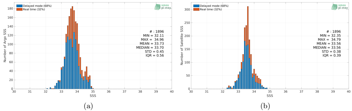
Figure 2: Histograms of SSS from Argo (a) and SMAP SSS L3 v4 - Monthly (RSS) (b) considering all match-up pairs per bins of 0.1 over the South China Sea Pi-MEP region and for the full satellite product period.
