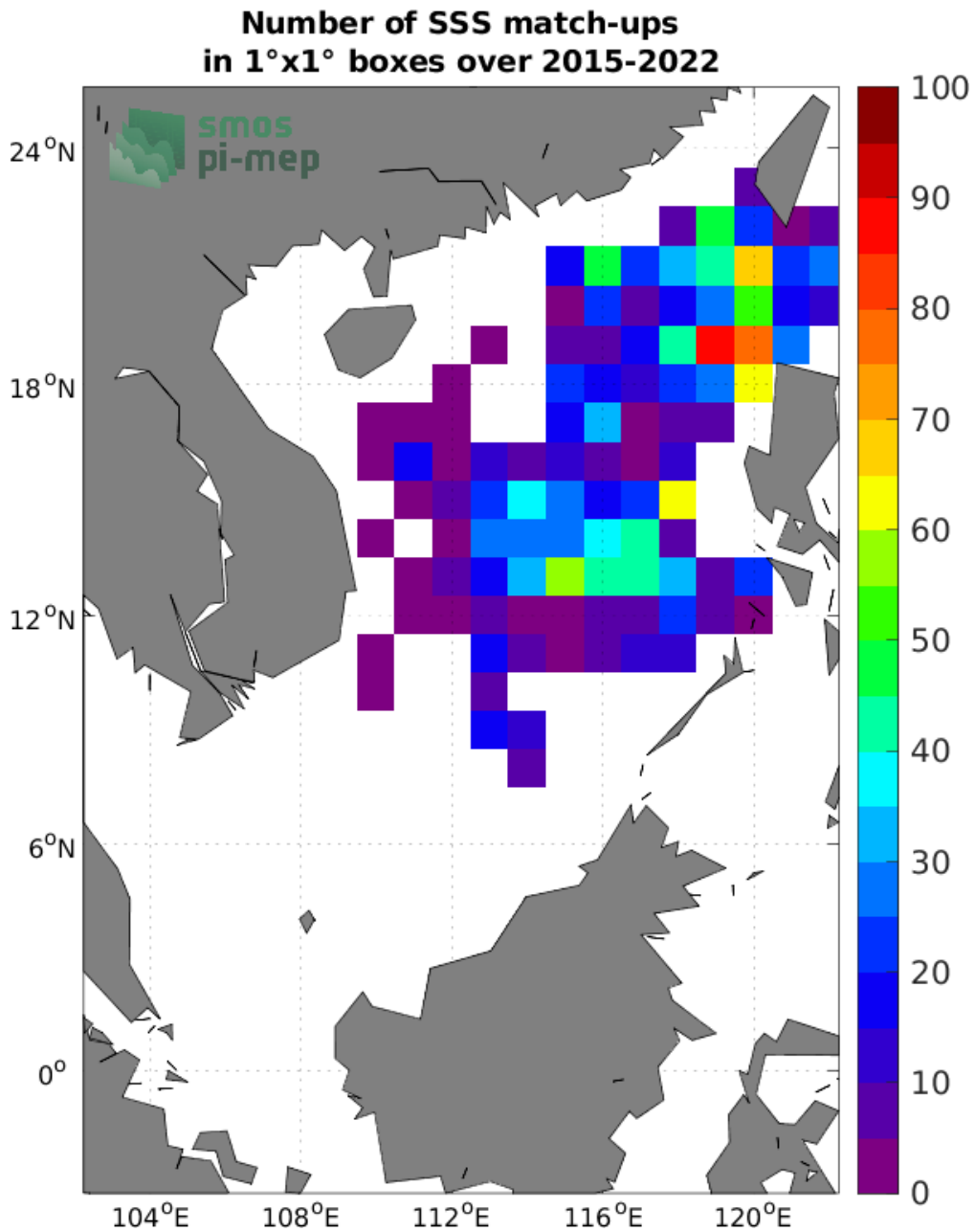
Figure 4: Number of SSS match-ups between Argo SSS and the SMAP SSS L3 v4 - Monthly (RSS) SSS product for the South China Sea Pi-MEP region over 1°x1° boxes and for the full satellite product period.
