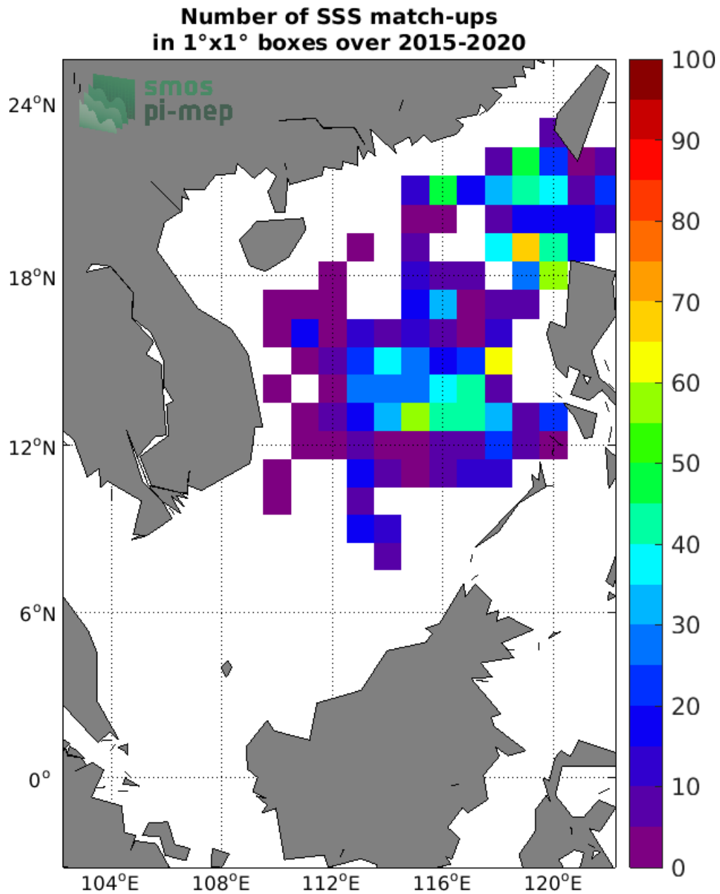
Figure 4: Number of SSS match-ups between Argo SSS and the SMAP SSS L3 v4 - Monthly (RSS) SSS product for the South China Sea Pi-MEP region over 1°x1° boxes and for the full satellite product period.
