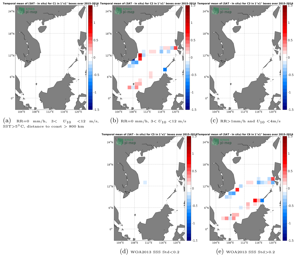
Figure 12: Temporal mean gridded over spatial boxes of size 1^\circ \times 1^\circ of \Delta SSS (SMAP-L3-RSS-V3-8DAY-RUNNING-40KM - TSG-SAMOS) for 5 different subdatasets corresponding to:RR=0 mm/h, 3 < U_{10} < 12 m/s, SST >5^\circ C, distance to coast > 800 km (a), RR=0 mm/h, 3 < U_{10} < 12 m/s (b), RR >1 mm/h and U_{10} < 4 m/s (c), WOA2013 SSS Std <0.2 (d), WOA2013 SSS Std >0.2 (e).
