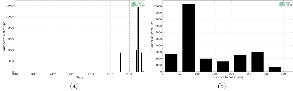
Figure 1: Number of match-ups between TSG-SAMOS and SMAP-L3-RSS-V3-8DAY-RUNNING-40KM SSS as a function of time (a) and as function of the distance to coast (b) over the South China Sea Pi-MEP region and for the full satellite product period.
