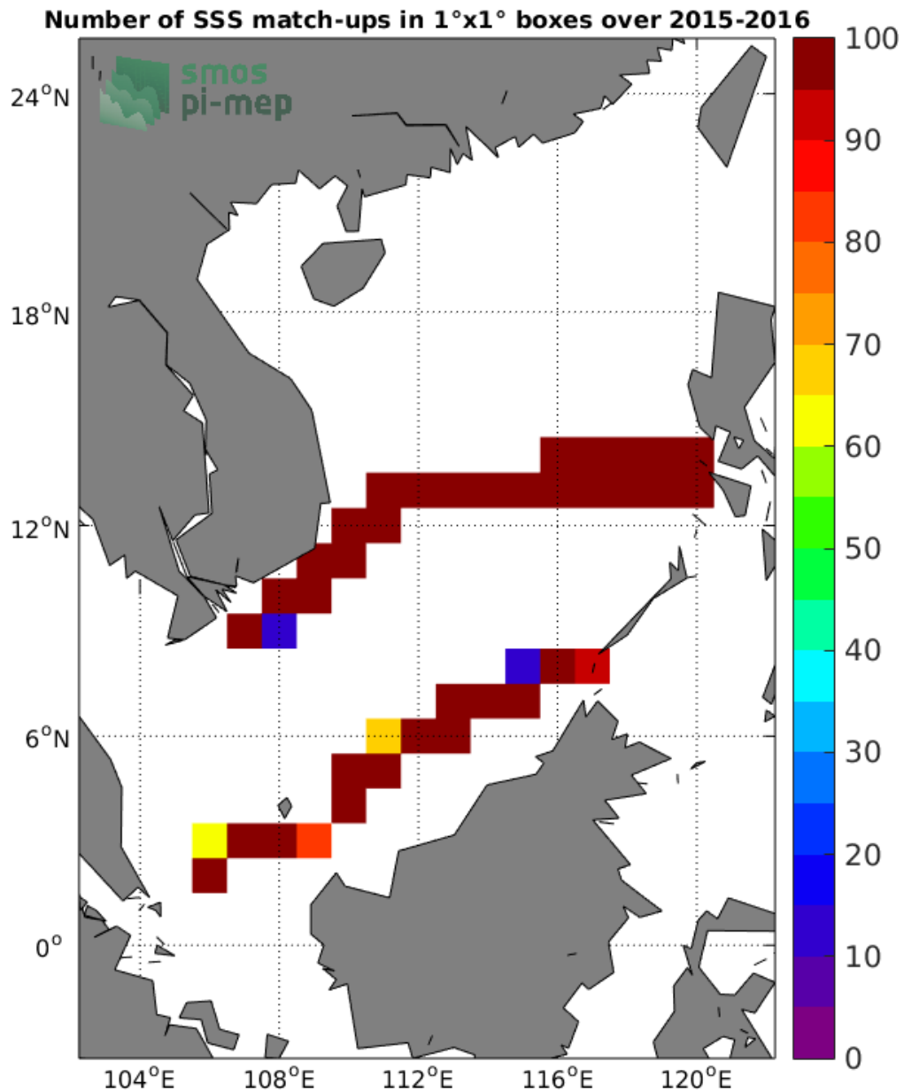
Figure 4: Number of SSS match-ups between TSG-SAMOS SSS and the SMAP-L3-RSS-V3-8DAY-RUNNING-40KM SSS product for the South China Sea Pi-MEP region over 1°x1° boxes and for the full satellite product period.
