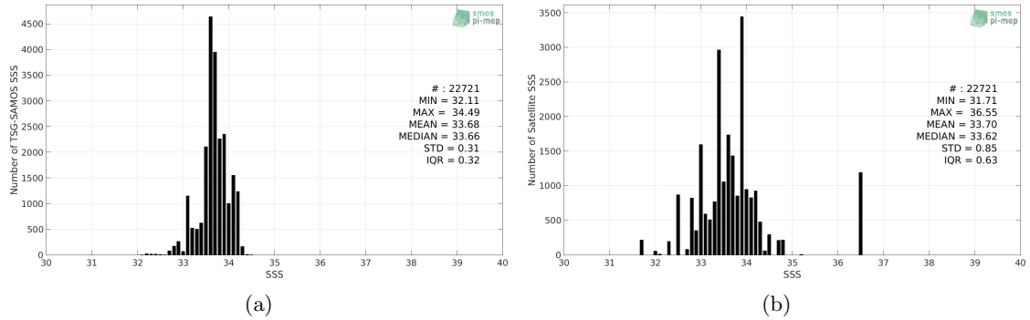
Figure 2: Histograms of SSS from TSG-SAMOS (a) and SMAP-L3-RSS-V3-8DAY-RUNNING-40KM (b) considering all match-up pairs per bins of 0.1 over the South China Sea Pi-MEP region and for the full satellite product period.
