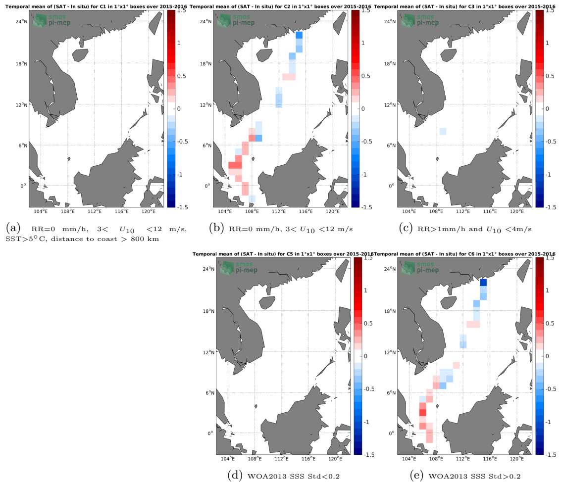
Figure 12: Temporal mean gridded over spatial boxes of size 1^\circ \times 1^\circ of \Delta SSS (SMAP-L3-RSS-V3-8DAY-RUNNING-40KM - TSG-LEGOS-DM) for 5 different subdatasets corresponding to:RR=0 mm/h, 3 < U_{10} < 12 m/s, SST >5^\circ C, distance to coast > 800 km (a), RR=0 mm/h, 3 < U_{10} < 12 m/s (b), RR >1 mm/h and U_{10} < 4 m/s (c), WOA2013 SSS Std <0.2 (d), WOA2013 SSS Std >0.2 (e).
