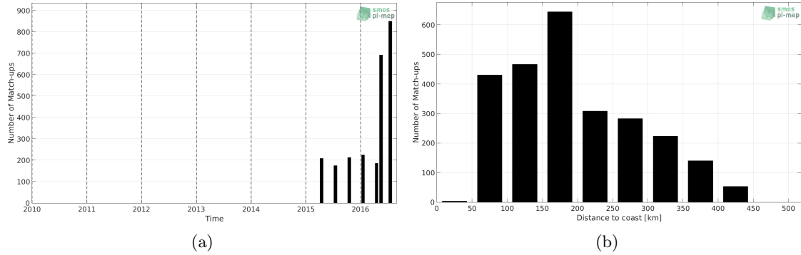
Figure 1: Number of match-ups between TSG-LEGOS-DM and SMAP-L3-RSS-V3-8DAY-RUNNING-40KM SSS as a function of time (a) and as function of the distance to coast (b) over the South China Sea Pi-MEP region and for the full satellite product period.
