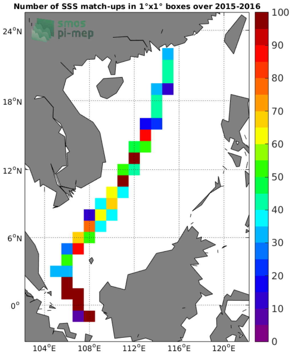
Figure 4: Number of SSS match-ups between TSG-LEGOS-DM SSS and the SMAP-L3-RSS-V3-8DAY-RUNNING-40KM SSS product for the South China Sea Pi-MEP region over 1°x1° boxes and for the full satellite product period.
