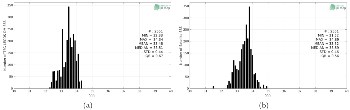
Figure 2: Histograms of SSS from TSG-LEGOS-DM (a) and SMAP-L3-RSS-V3-8DAY-RUNNING-40KM (b) considering all match-up pairs per bins of 0.1 over the South China Sea Pi-MEP region and for the full satellite product period.
