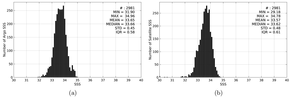
Figure 2: Histograms of SSS from Argo (a) and SMAP-L3-RSS-V2-8DAY-RUNNING-70KM (b) considering all match-up pairs per bins of 0.1 over the South China Sea Pi-MEP region and for the full satellite product period.
