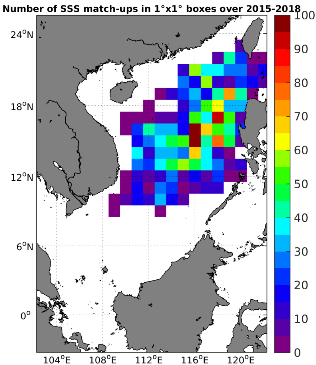
Figure 4: Number of SSS match-ups between Argo SSS and the SMAP-L3-RSS-V2-8DAY-RUNNING-70KM SSS product for the South China Sea Pi-MEP region over 1°x1° boxes and for the full satellite product period.
