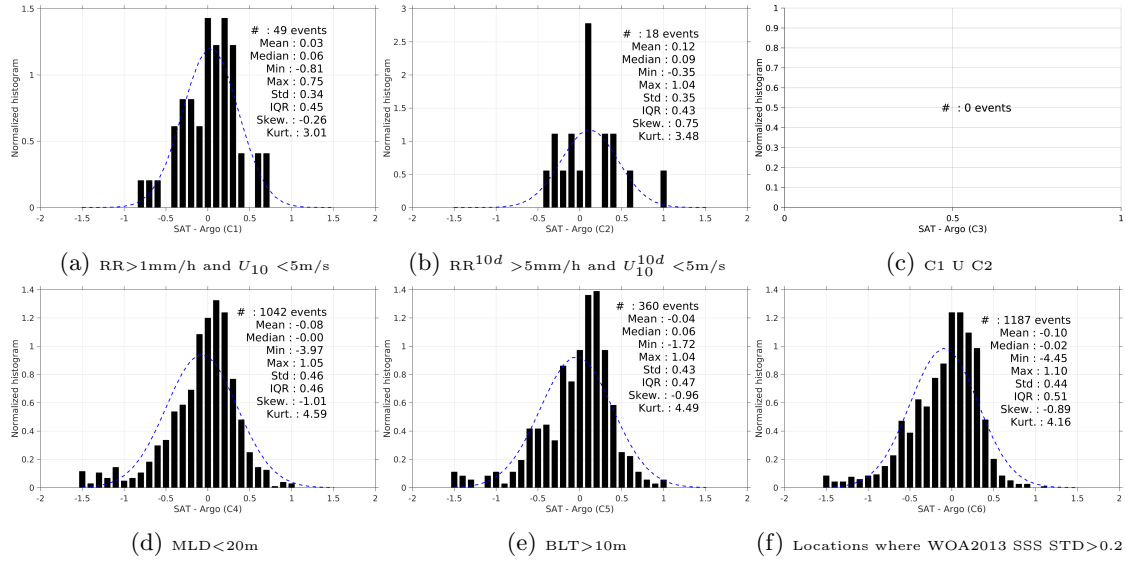
Figure 13: Normalized histogram of \Delta SSS (SMAP-L3-RSS-V2-8DAY-RUNNING-70KM - Argo) for 6 different subdatasets corresponding to: RR > 1mm/h and U_{10} < 5 m/s (a), RR^{10d} > 5 mm/h and U_{10}^{10d} < 5 m/s (b), C1 U C2 (c), MLD < 20m (d), BLT > 10m (e), Locations where WOA2013 SSS STD > 0.2 (f).
