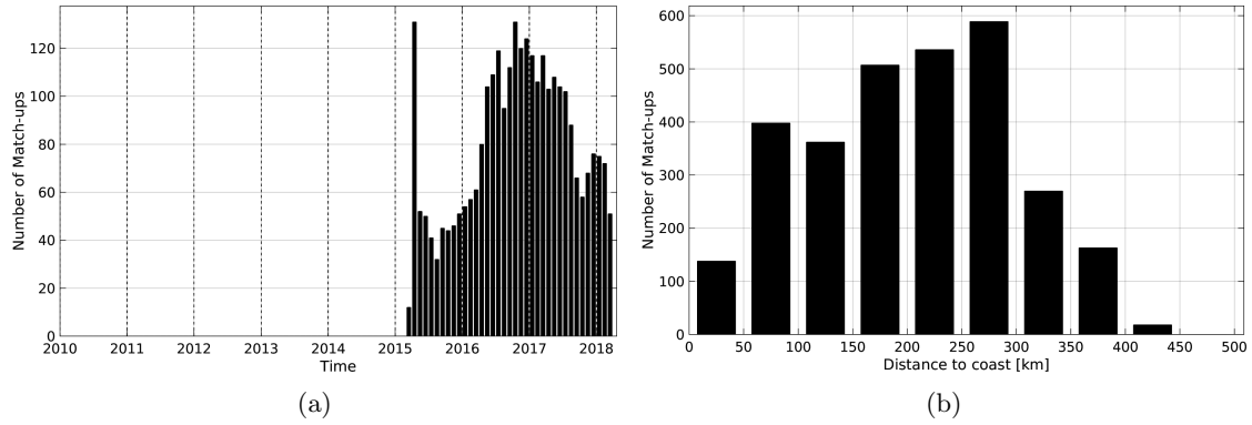
Figure 1: Number of match-ups between Argo and SMAP-L3-RSS-V2-8DAY-RUNNING-70KM SSS as a function of time (a) and as function of the distance to coast (b) over the South China Sea Pi-MEP region and for the full satellite product period.
