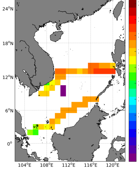
(c) MEAN(TSG-SAMOS SSS)
