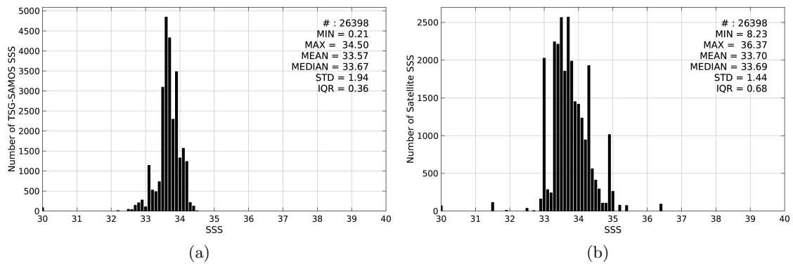
Figure 2: Histograms of SSS from TSG-SAMOS (a) and SMAP-L3-RSS-V2-MONTHLY-0.25DEG-40KM (b) considering all match-up pairs per bins of 0.1 over the South China Sea Pi-MEP region and for the full satellite product period.
