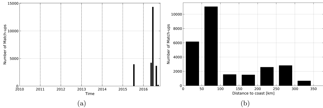
Figure 1: Number of match-ups between TSG-SAMOS and SMAP-L3-RSS-V2-MONTHLY-0.25DEG-40KM SSS as a function of time (a) and as function of the distance to coast (b) over the South China Sea Pi-MEP region and for the full satellite product period.
