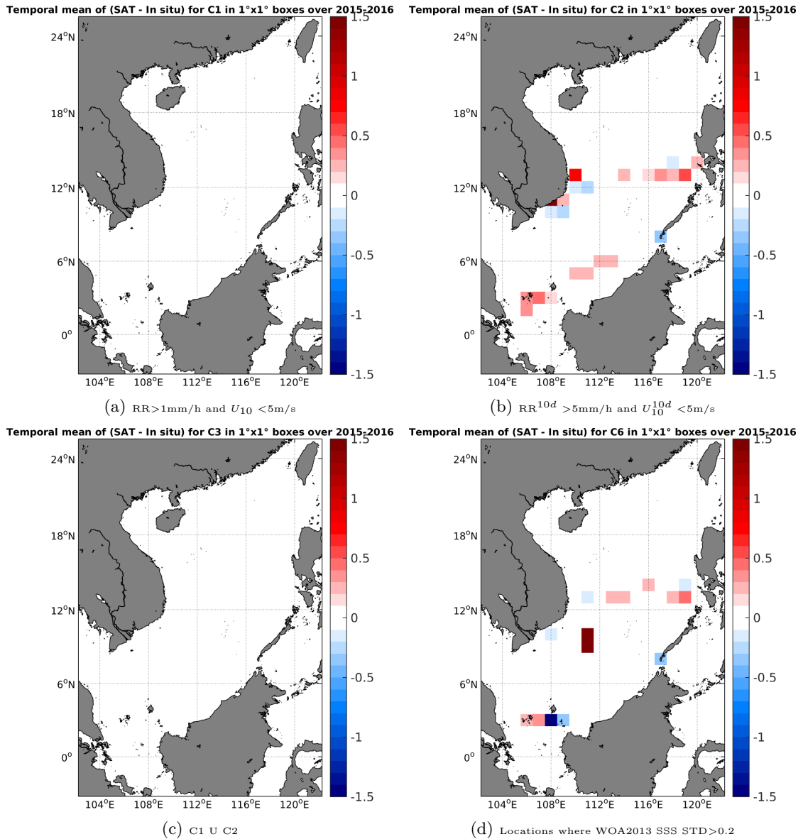
Figure 12: Temporal mean gridded over spatial boxes of size 1°x1° of \Delta SSS (SMAP-L3-RSS-V2-MONTHLY-0.25DEG-40KM - TSG-SAMOS) for 4 different subdatasets corresponding to: RR > 1\text{mm/h} and U_{10} < 5\text{m/s} (a), RR^{10d} > 5\text{mm/h} and U_{10}^{10d} < 5\text{m/s} (b), C1 U C2 (c), Locations where WOA2013 SSS STD > 0.2 (d).
