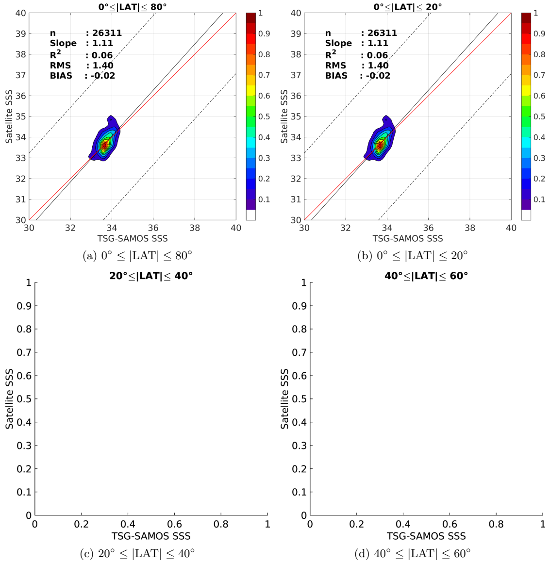
Figure 9: Contour maps of the concentration of SMAP-L3-RSS-V2-MONTHLY-0.25DEG-40KM SSS (y-axis) versus TSG-SAMOS SSS (x-axis) at match-up pairs for different latitude bands. For each plot, the red line shows x=y . The black thin and dashed lines indicate a linear fit through the data cloud and the \pm 95\% confidence levels, respectively. The number match-up pairs n , the slope and R^2 coefficient of the linear fit, the root mean square (RMS) and the mean bias between satellite and in situ data are indicated for each latitude band in each plots.
