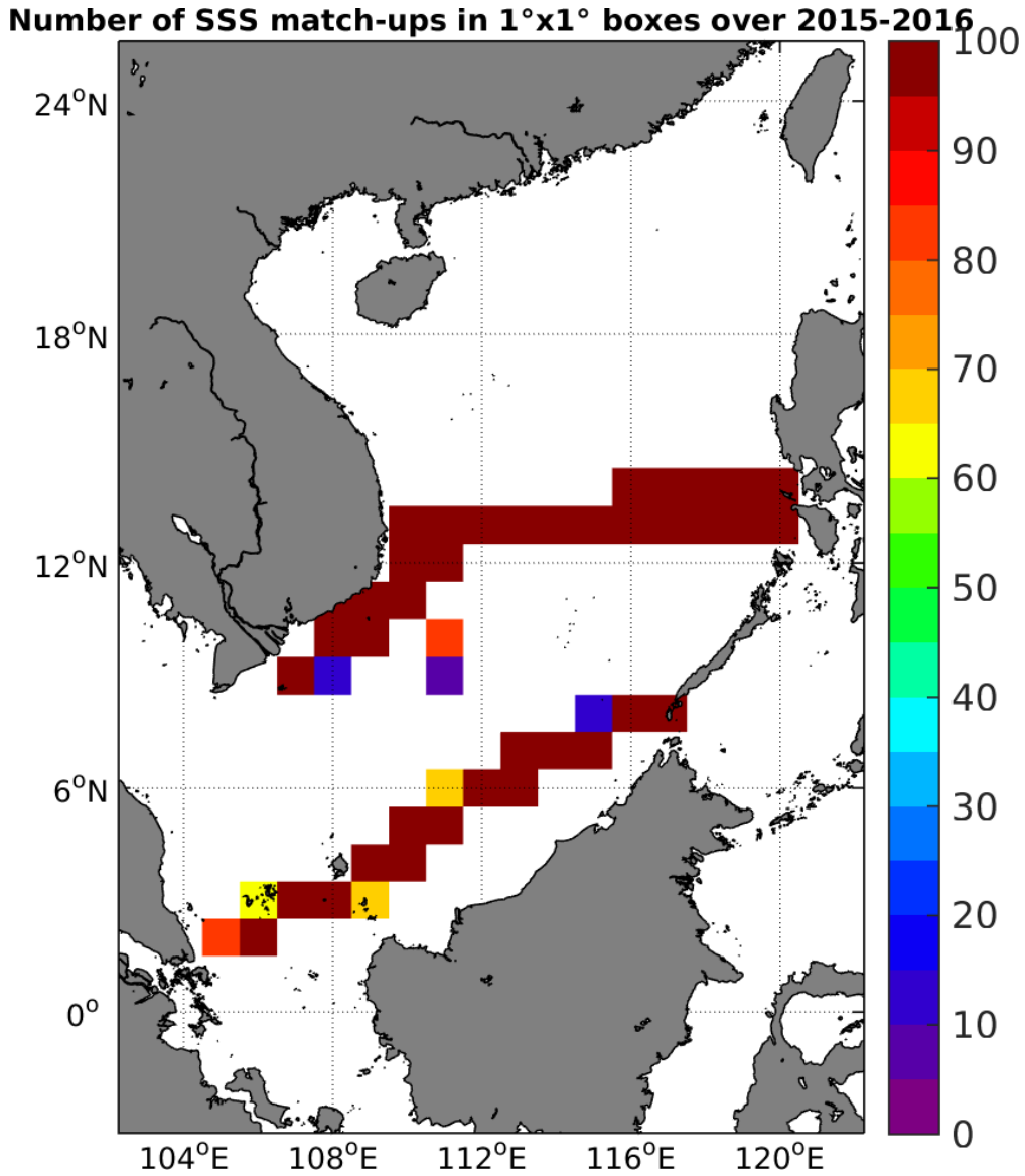
Figure 4: Number of SSS match-ups between TSG-SAMOS SSS and the SMAP-L3-RSS-V2-MONTHLY-0.25DEG-40KM SSS product for the South China Sea Pi-MEP region over 1°x1° boxes and for the full satellite product period.
