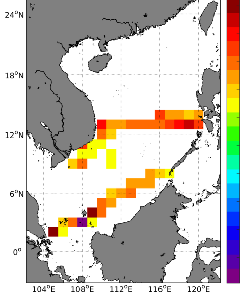
(a) MEAN(Satellite SSS)
