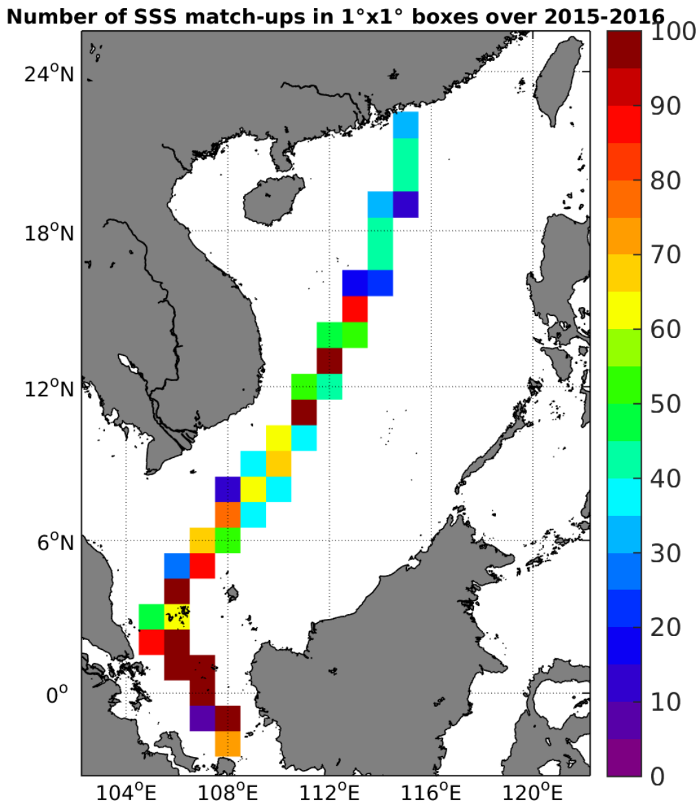
Figure 4: Number of SSS match-ups between TSG-LEGOS-DM SSS and the SMAP-L3-RSS-V2-MONTHLY-0.25DEG-40KM SSS product for the South China Sea Pi-MEP region over 1°x1° boxes and for the full satellite product period.
