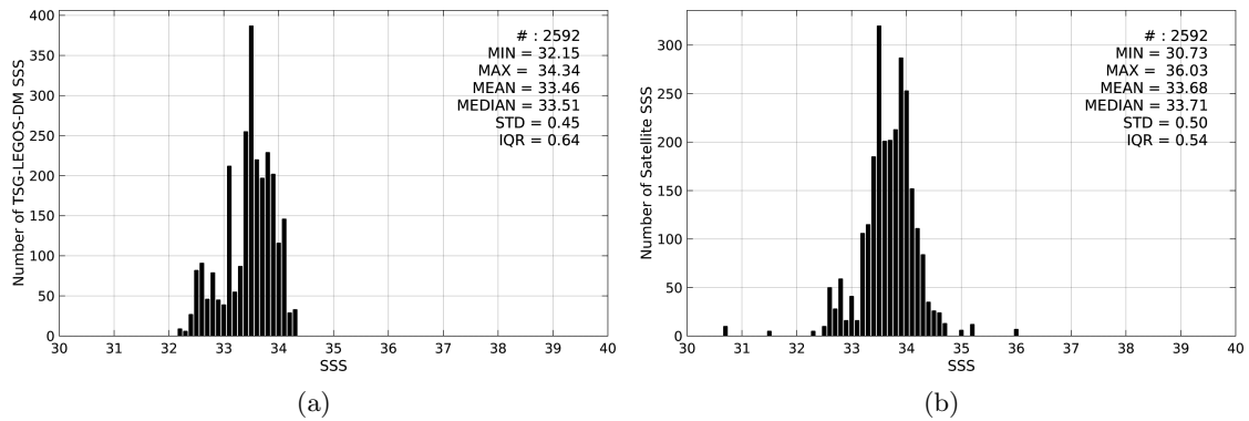
Figure 2: Histograms of SSS from TSG-LEGOS-DM (a) and SMAP-L3-RSS-V2-MONTHLY-0.25DEG-40KM (b) considering all match-up pairs per bins of 0.1 over the South China Sea Pi-MEP region and for the full satellite product period.
