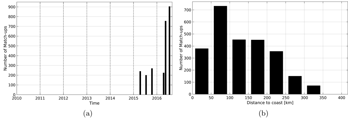
Figure 1: Number of match-ups between TSG-LEGOS-DM and SMAP-L3-RSS-V2-MONTHLY-0.25DEG-40KM SSS as a function of time (a) and as function of the distance to coast (b) over the South China Sea Pi-MEP region and for the full satellite product period.
