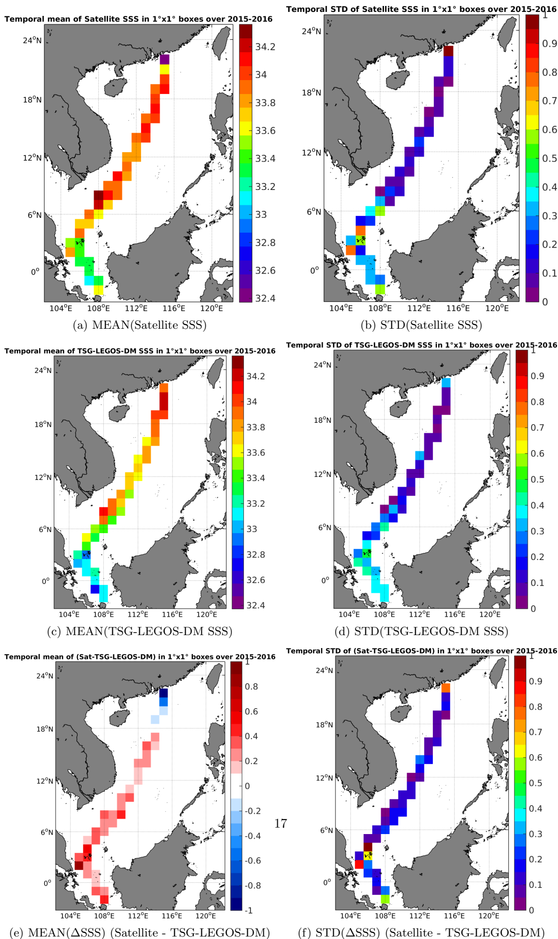
Figure 6: Temporal mean (left) and STD (right) of SSS from SMAP-L3-RSS-V2-MONTHLY-0.25DEG-40KM (top), TSG-LEGOS-DM (middle), and of \Delta SSS (Satellite - TSG-LEGOS-DM). Only match-up pairs are used to generate these maps.
