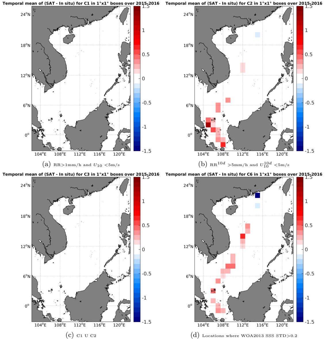
Figure 12: Temporal mean gridded over spatial boxes of size 1°x1° of \Delta SSS (SMAP-L3-RSS-V2-MONTHLY-0.25DEG-40KM - TSG-LEGOS-DM) for 4 different subdatasets corresponding to: RR > 1\text{mm/h} and U_{10} < 5\text{m/s} (a), RR^{10d} > 5\text{mm/h} and U_{10}^{10d} < 5\text{m/s} (b), C1 U C2 (c), Locations where WOA2013 SSS STD > 0.2 (d).
