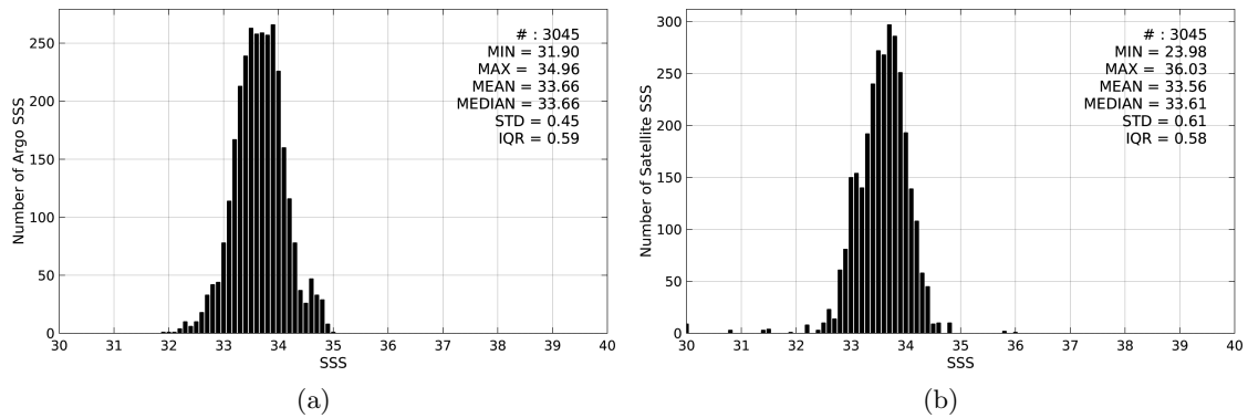
Figure 2: Histograms of SSS from Argo (a) and SMAP-L3-RSS-V2-MONTHLY-0.25DEG-40KM (b) considering all match-up pairs per bins of 0.1 over the South China Sea Pi-MEP region and for the full satellite product period.
