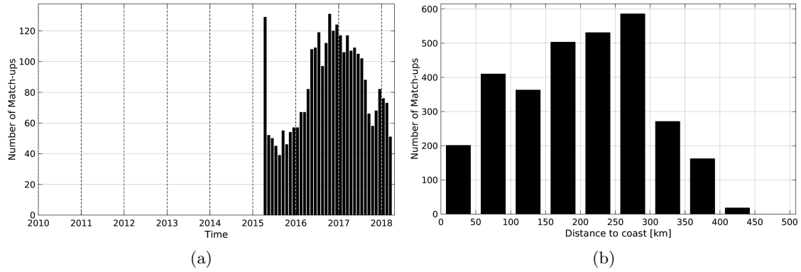
Figure 1: Number of match-ups between Argo and SMAP-L3-RSS-V2-MONTHLY-0.25DEG-40KM SSS as a function of time (a) and as function of the distance to coast (b) over the South China Sea Pi-MEP region and for the full satellite product period.
