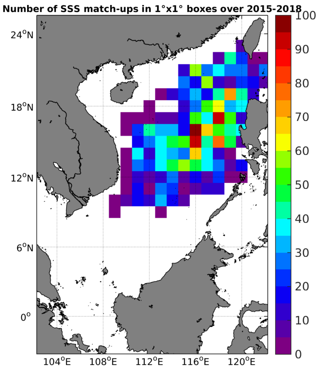
Figure 4: Number of SSS match-ups between Argo SSS and the SMAP-L3-RSS-V2-MONTHLY-0.25DEG-40KM SSS product for the South China Sea Pi-MEP region over 1°x1° boxes and for the full satellite product period.
