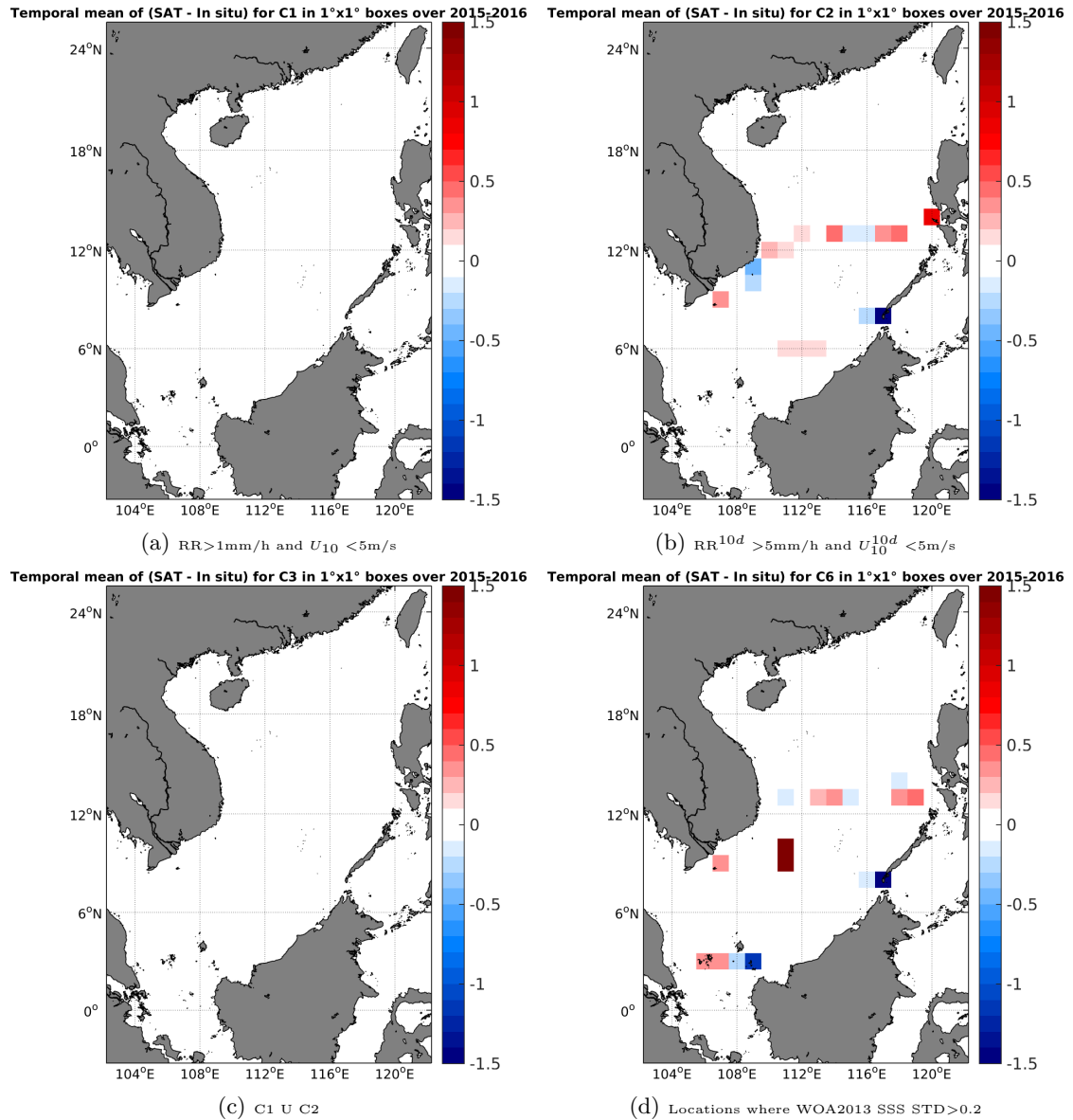
Figure 12: Temporal mean gridded over spatial boxes of size 1^\circ \times 1^\circ of \Delta SSS (SMAP-L3-RSS-V2-MONTHLY-70KM - TSG-SAMOS) for 4 different subdatasets corresponding to:RR > 1 mm/h and U_{10} < 5 m/s (a), RR 10d > 5 mm/h and U_{10}^{10d} < 5 m/s (b), C1 U C2 (c),Locations where WOA2013 SSS STD > 0.2 (d).
