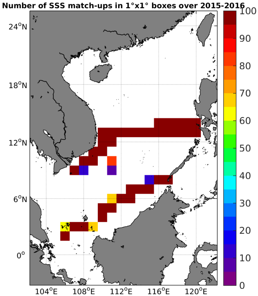
Figure 4: Number of SSS match-ups between TSG-SAMOS SSS and the SMAP-L3-RSS-V2-MONTHLY-70KM SSS product for the South China Sea Pi-MEP region over 1°x1° boxes and for the full satellite product period.
