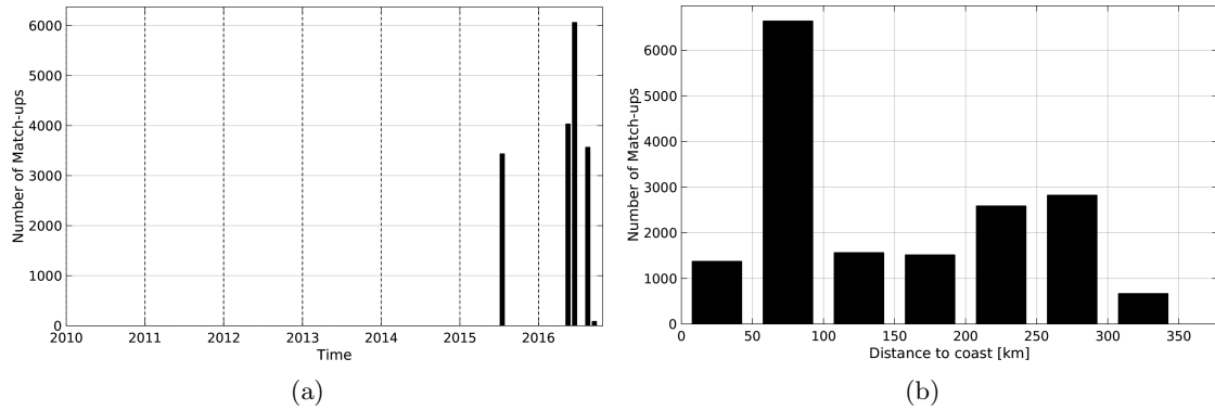
Figure 1: Number of match-ups between TSG-SAMOS and SMAP-L3-RSS-V2-MONTHLY-70KM SSS as a function of time (a) and as function of the distance to coast (b) over the South China Sea Pi-MEP region and for the full satellite product period.
