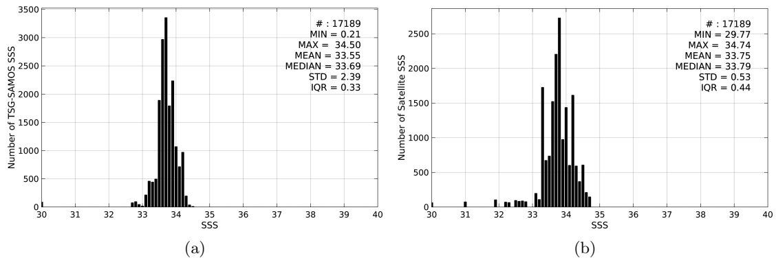
Figure 2: Histograms of SSS from TSG-SAMOS (a) and SMAP-L3-RSS-V2-MONTHLY-70KM (b) considering all match-up pairs per bins of 0.1 over the South China Sea Pi-MEP region and for the full satellite product period.
