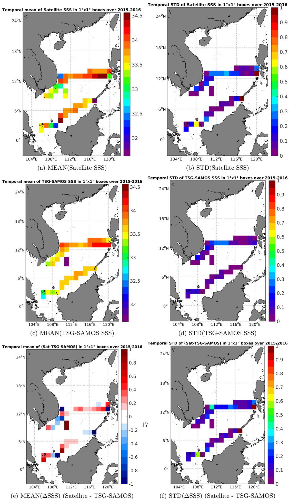
Figure 6: Temporal mean (left) and STD (right) of SSS from SMAP-L3-RSS-V2-MONTHLY-
