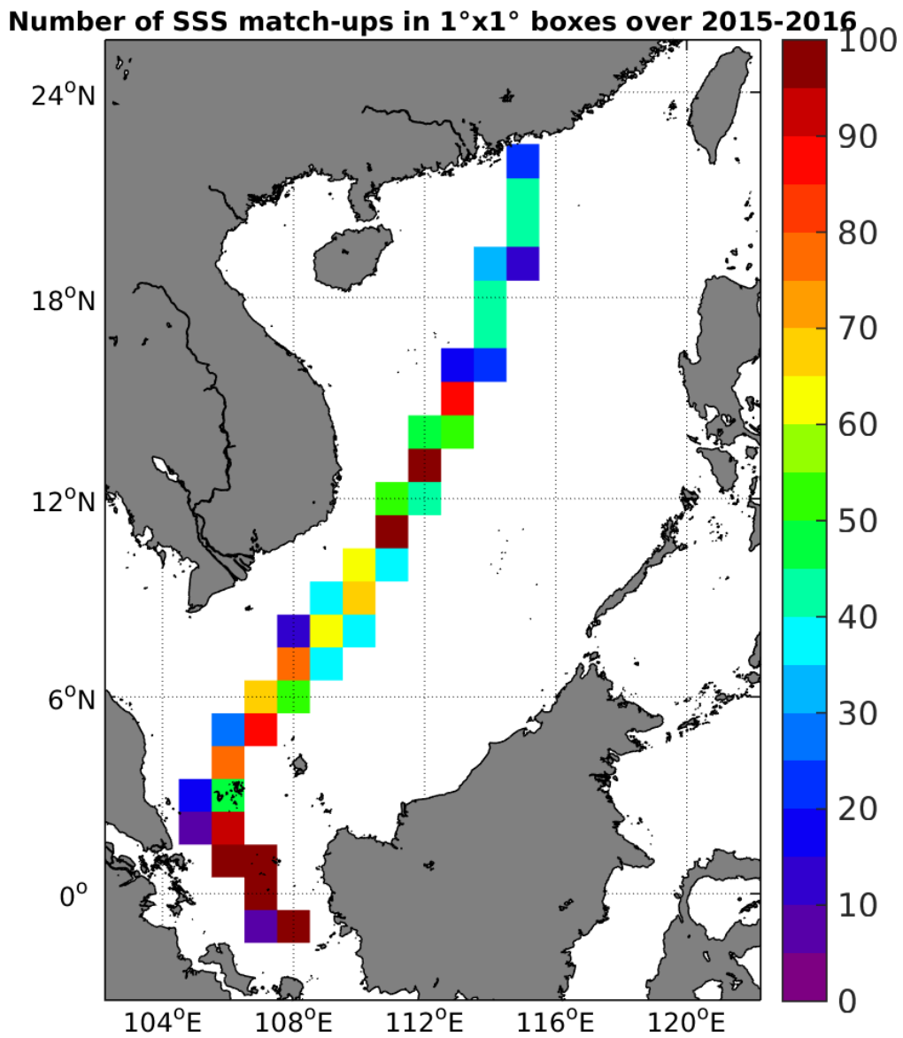
Figure 4: Number of SSS match-ups between TSG-LEGOS-DM SSS and the SMAP-L3-RSS-V2-MONTHLY-70KM SSS product for the South China Sea Pi-MEP region over 1°x1° boxes and for the full satellite product period.
