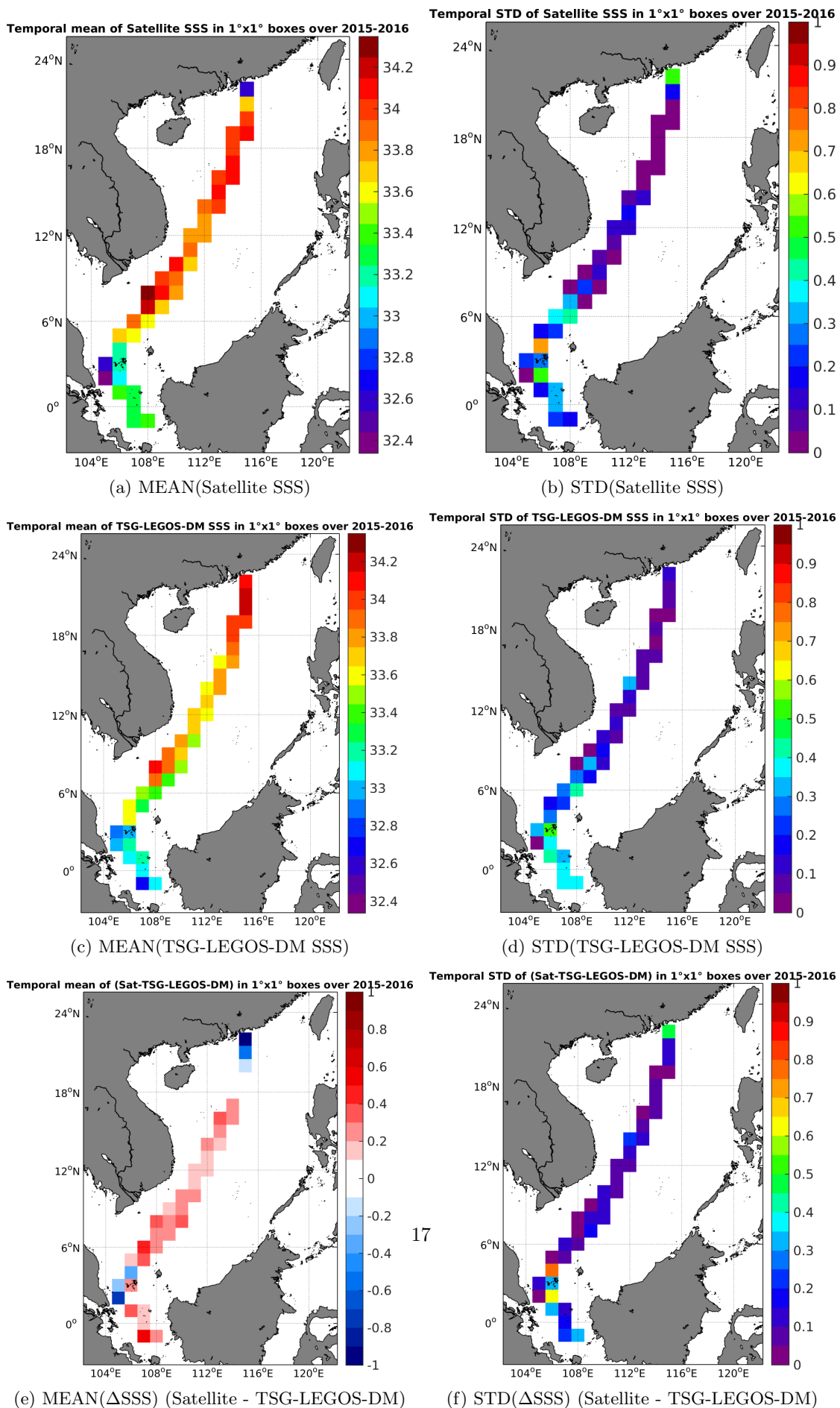
Figure 6: Temporal mean (left) and STD (right) of SSS from SMAP-L3-RSS-V2-MONTHLY-70KM (top), TSG-LEGOS-DM (middle), and of \Delta SSS (Satellite - TSG-LEGOS-DM). Only match-up pairs are used to generate these maps.
