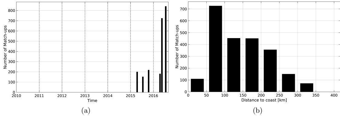
Figure 1: Number of match-ups between TSG-LEGOS-DM and SMAP-L3-RSS-V2-MONTHLY-70KM SSS as a function of time (a) and as function of the distance to coast (b) over the South China Sea Pi-MEP region and for the full satellite product period.
