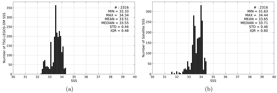
Figure 2: Histograms of SSS from TSG-LEGOS-DM (a) and SMAP-L3-RSS-V2-MONTHLY-70KM (b) considering all match-up pairs per bins of 0.1 over the South China Sea Pi-MEP region and for the full satellite product period.
