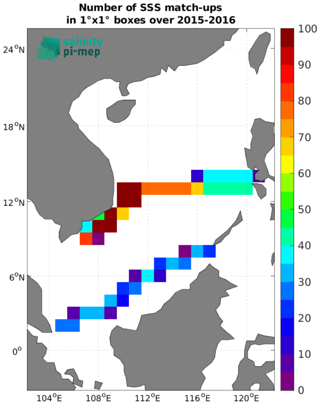
Figure 5: Number of SSS match-ups between TSG (SAMOS) SSS and the SMAP SSS L3 v5.0 - 8-Day running (JPL) SSS product for the South China Sea Pi-MEP region over 1^\circ \times 1^\circ boxes and for the full satellite product period.
