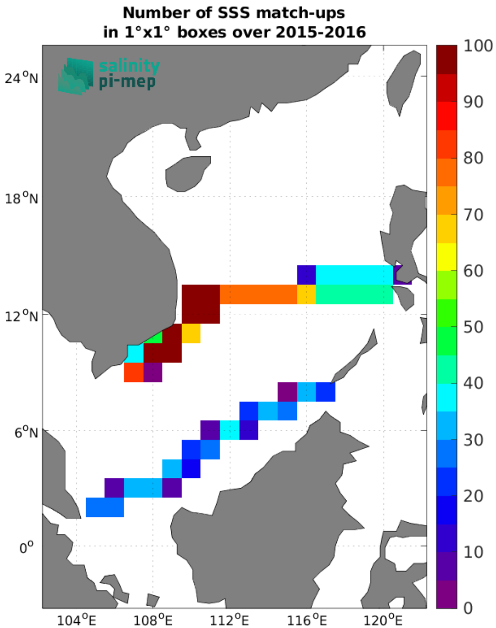
Figure 5: Number of SSS match-ups between TSG (SAMOS) SSS and the SMAP SSS L3 v5.0 - 8-Day running (JPL) SSS product for the South China Sea Pi-MEP region over 1°×1° boxes and for the full satellite product period.
