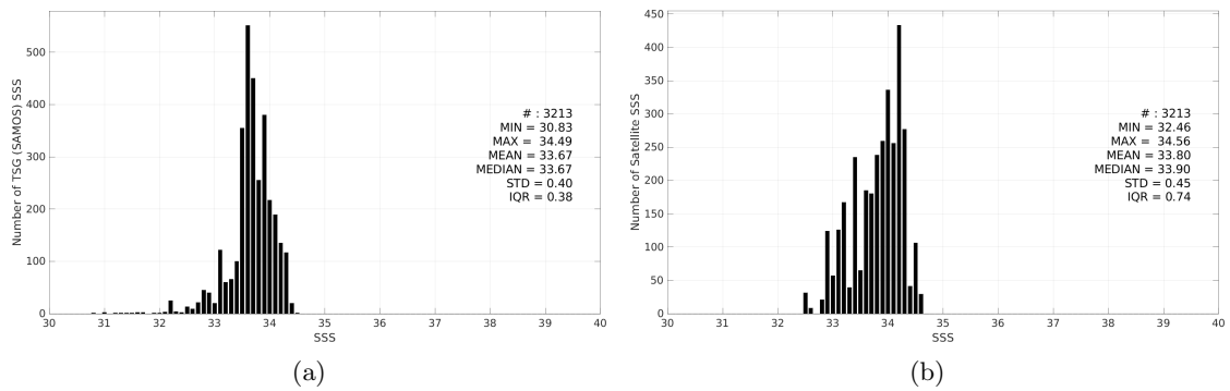
Figure 3: Histograms of SSS from TSG (SAMOS) (a) and SMAP SSS L3 v5.0 - 8-Day running (JPL) (b) considering all match-up pairs per bins of 0.1 over the South China Sea Pi-MEP region and for the full satellite product period.
