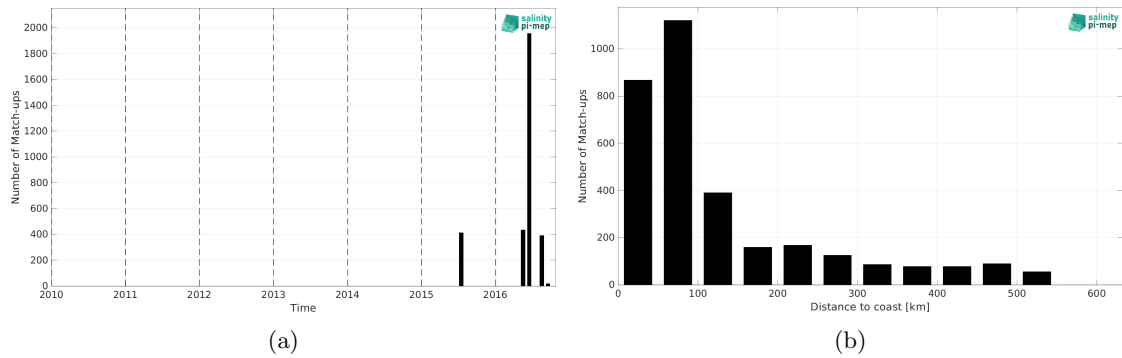
Figure 2: Number of match-ups between TSG (SAMOS) and SMAP SSS L3 v5.0 - 8-Day running (JPL) SSS as a function of time (a) and as function of the distance to coast (b) over the South China Sea Pi-MEP region and for the full satellite product period.
