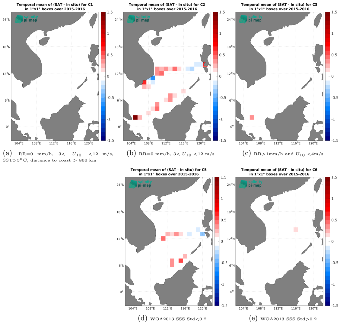
Figure 14: Temporal mean gridded over spatial boxes of size 1^\circ \times 1^\circ of \Delta SSS (SMAP SSS L3 v5.0 - 8-Day running (JPL) - TSG (SAMOS)) for 5 different subdatasets corresponding to: RR=0 mm/h, 3 < U_{10} < 12 m/s, SST > 5°C, distance to coast > 800 km (a), RR=0 mm/h, 3 < U_{10} < 12 m/s (b), RR > 1mm/h and U_{10} < 4 m/s (c), WOA2013 SSS Std < 0.2 (d), WOA2013 SSS Std > 0.2 (e).
