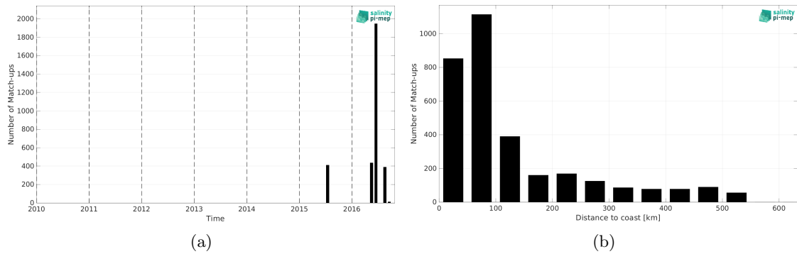
Figure 1: Number of match-ups between TSG (SAMOS) and SMAP SSS L3 v5.0 - 8-Day running (JPL) SSS as a function of time (a) and as function of the distance to coast (b) over the South China Sea Pi-MEP region and for the full satellite product period.
