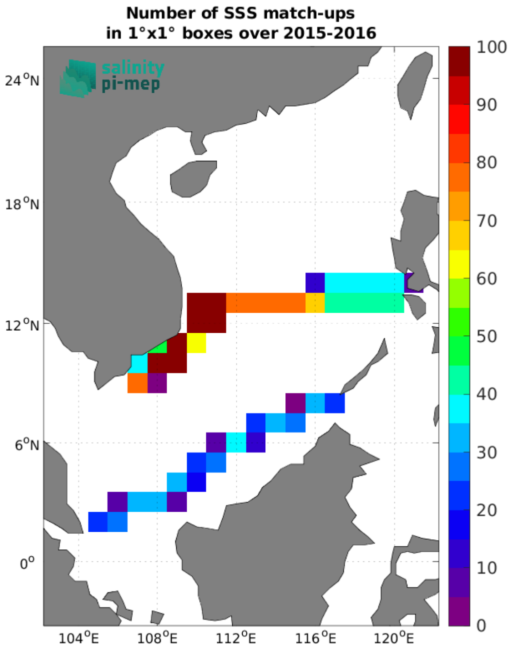
Figure 4: Number of SSS match-ups between TSG (SAMOS) SSS and the SMAP SSS L3 v5.0 - 8-Day running (JPL) SSS product for the South China Sea Pi-MEP region over 1^\circ \times 1^\circ boxes and for the full satellite product period.
