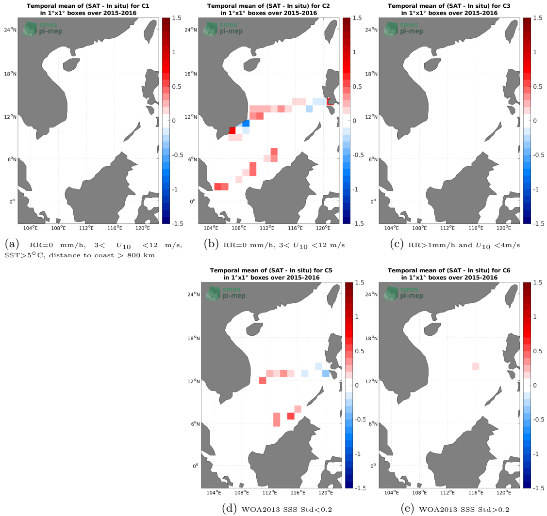
Figure 12: Temporal mean gridded over spatial boxes of size 1^\circ \times 1^\circ of \Delta SSS (SMAP SSS L3 v5.0 - 8-Day running (JPL) - TSG (SAMOS)) for 5 different subdatasets corresponding to: RR=0 mm/h, 3 < U_{10} < 12 m/s, SST > 5°C, distance to coast > 800 km (a), RR=0 mm/h, 3 < U_{10} < 12 m/s (b), RR > 1mm/h and U_{10} < 4 m/s (c), WOA2013 SSS Std < 0.2 (d), WOA2013 SSS Std > 0.2 (e).
