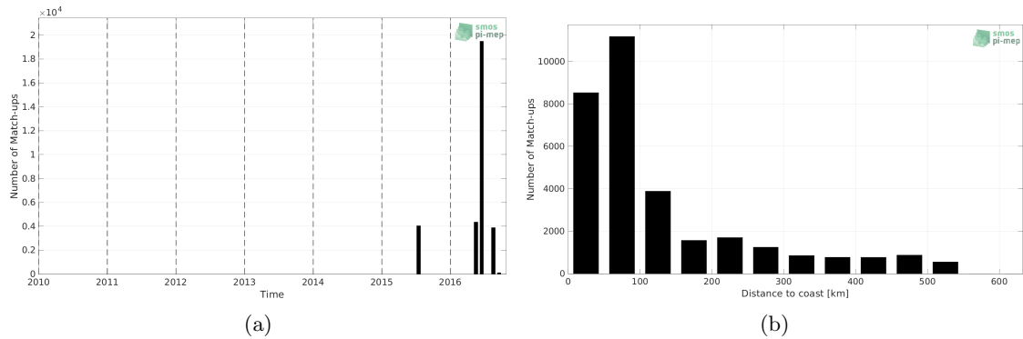
Figure 1: Number of match-ups between TSG (SAMOS) and SMAP SSS L3 v5.0 - 8-Day running (JPL) SSS as a function of time (a) and as function of the distance to coast (b) over the South China Sea Pi-MEP region and for the full satellite product period.
