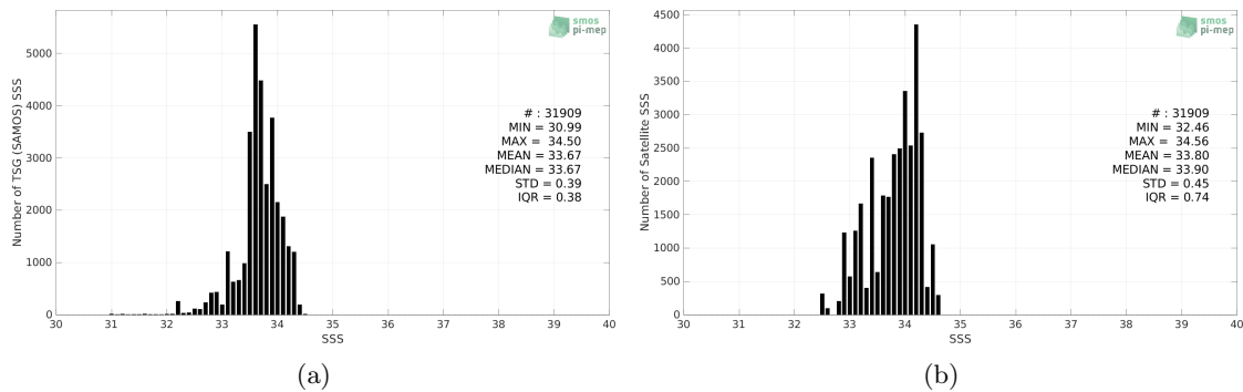
Figure 2: Histograms of SSS from TSG (SAMOS) (a) and SMAP SSS L3 v5.0 - 8-Day running (JPL) (b) considering all match-up pairs per bins of 0.1 over the South China Sea Pi-MEP region and for the full satellite product period.
