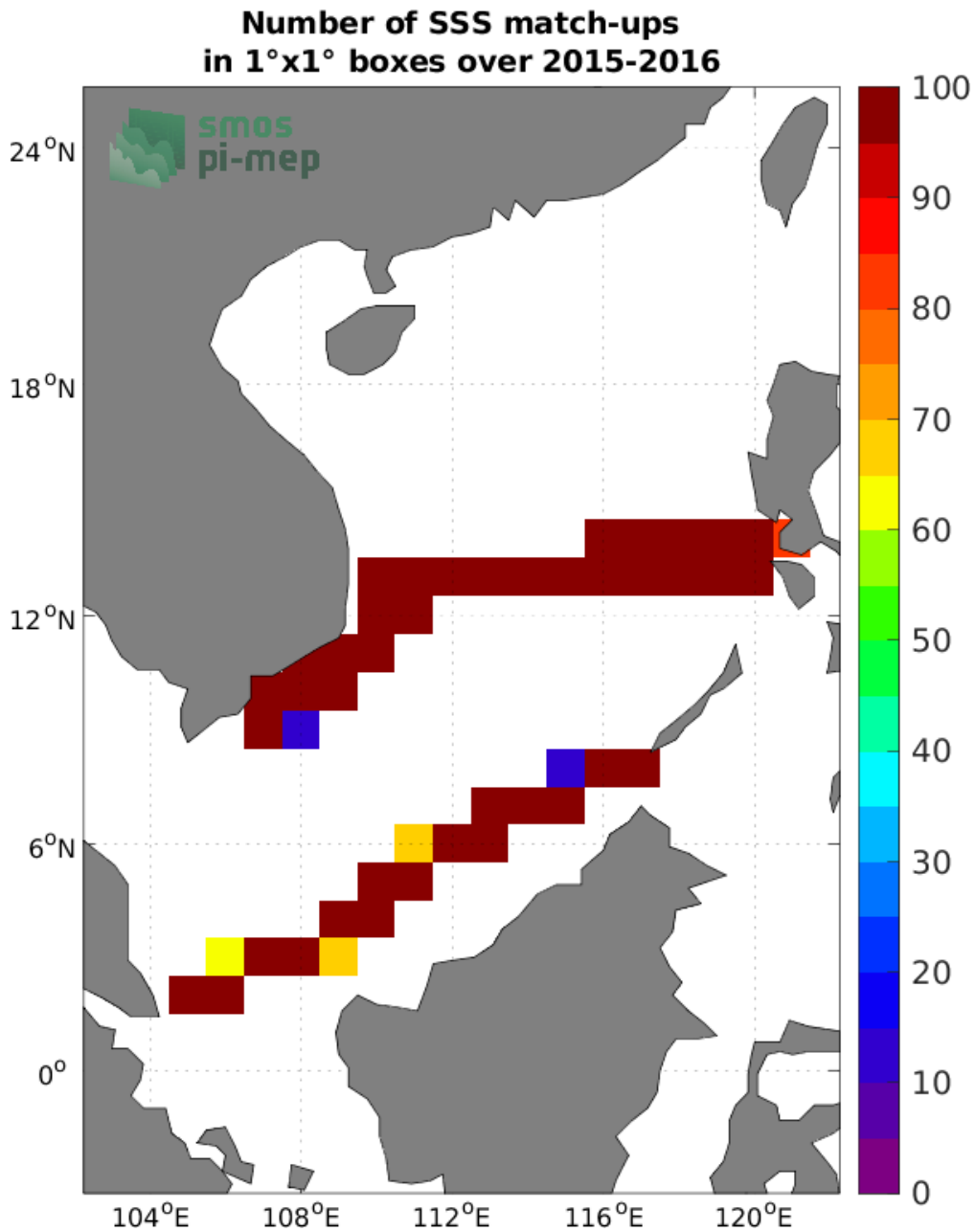
Figure 4: Number of SSS match-ups between TSG (SAMOS) SSS and the SMAP SSS L3 v5.0 - 8-Day running (JPL) SSS product for the South China Sea Pi-MEP region over 1°x1° boxes and for the full satellite product period.
