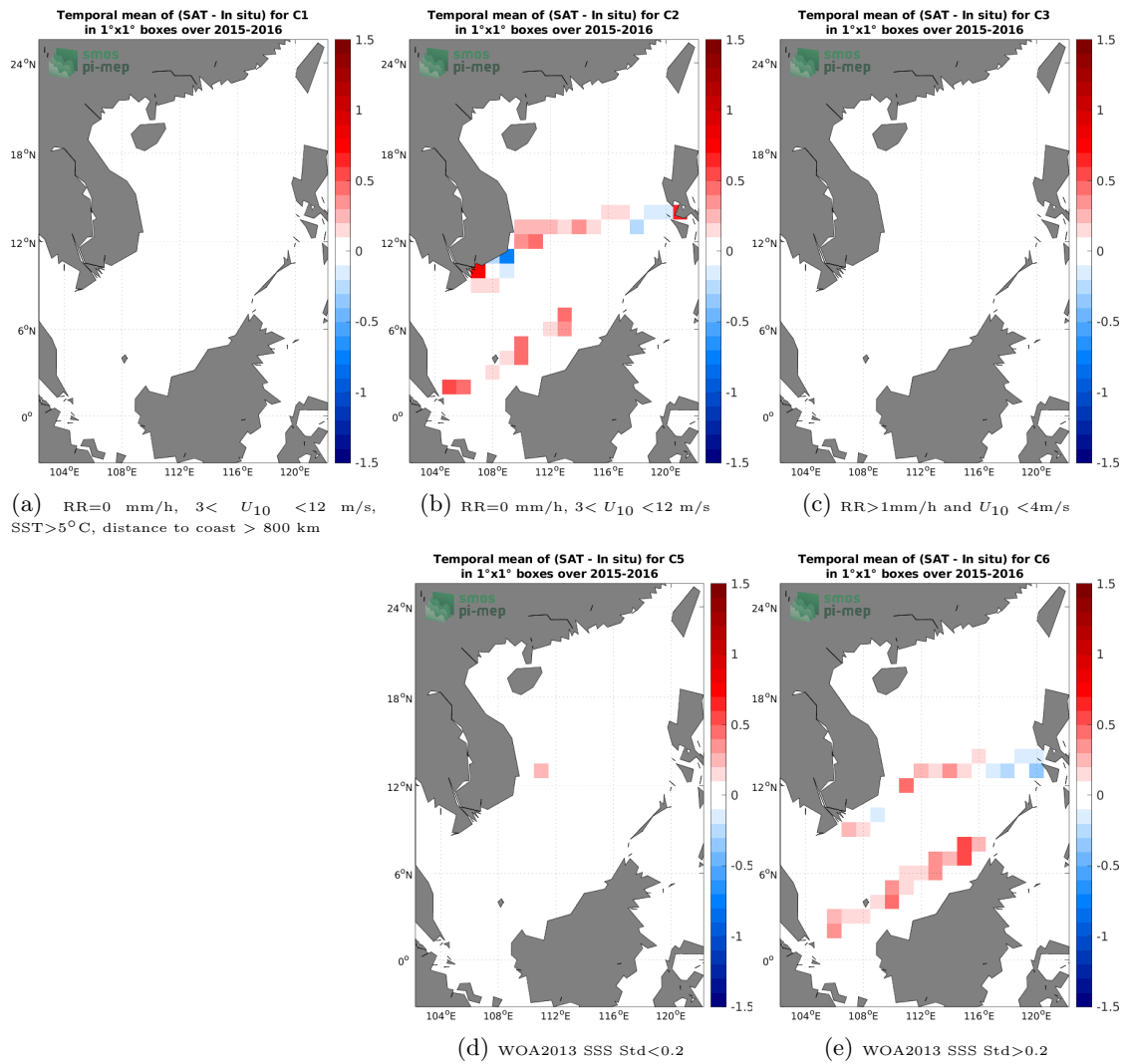
Figure 12: Temporal mean gridded over spatial boxes of size 1^\circ \times 1^\circ of \Delta\text{SSS} (SMAP SSS L3 v5.0 - 8-Day running (JPL) - TSG (SAMOS)) for 5 different subdatasets corresponding to: RR=0 mm/h, 3 < U_{10} < 12 m/s, SST > 5^\circ\text{C} , distance to coast > 800 km (a), RR=0 mm/h, 3 < U_{10} < 12 m/s (b), RR > 1 mm/h and U_{10} < 4 m/s (c), WOA2013 SSS Std <0.2 (d), WOA2013 SSS Std >0.2 (e).
