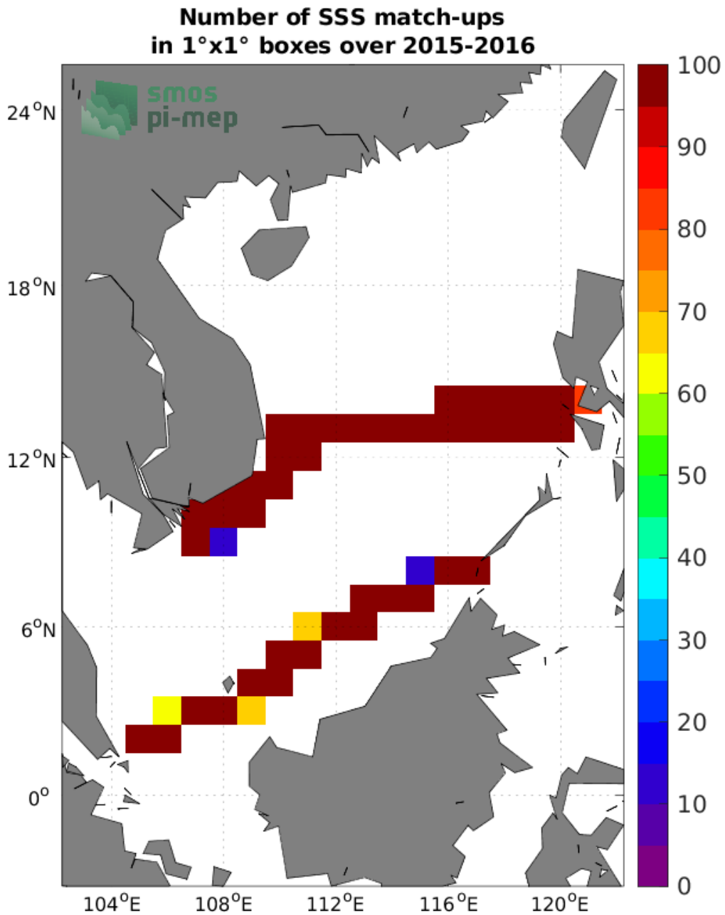
Figure 4: Number of SSS match-ups between TSG (SAMOS) SSS and the SMAP SSS L3 v5.0 - 8-Day running (JPL) SSS product for the South China Sea Pi-MEP region over 1°×1° boxes and for the full satellite product period.
