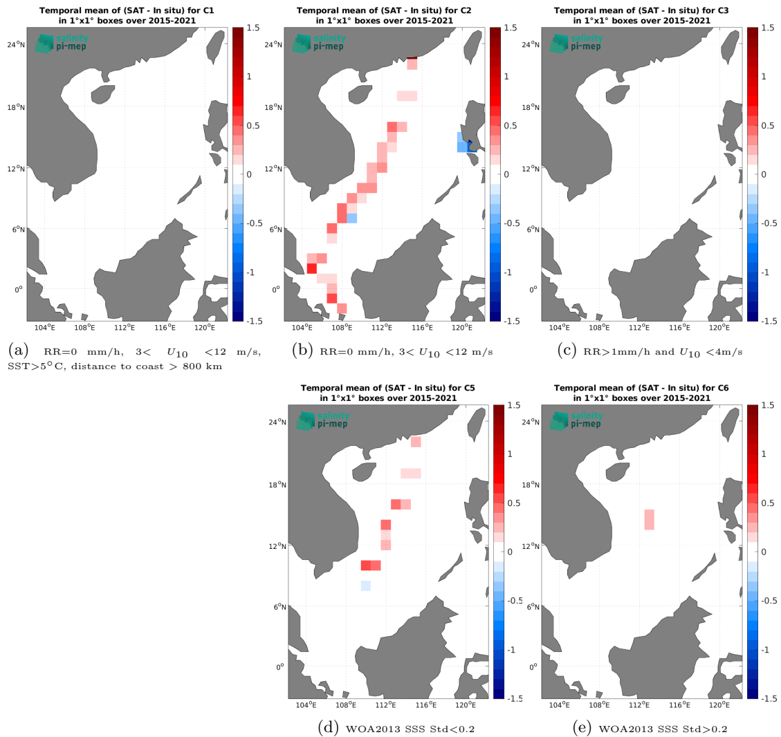
Figure 14: Temporal mean gridded over spatial boxes of size 1^\circ \times 1^\circ of \Delta SSS (SMAP SSS L3 v5.0 - 8-Day running (JPL) - TSG (LEGOS-DM)) for 5 different subdatasets corresponding to:RR=0 mm/h, 3 < U_{10} < 12 m/s, SST>5°C, distance to coast > 800 km (a), RR=0 mm/h, 3 < U_{10} < 12 m/s (b), RR>1mm/h and U_{10} < 4 m/s (c), WOA2013 SSS Std<0.2 (d), WOA2013 SSS Std>0.2 (e).
