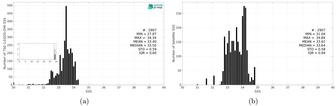
Figure 3: Histograms of SSS from TSG (LEGOS-DM) (a) and SMAP SSS L3 v5.0 - 8-Day running (JPL) (b) considering all match-up pairs per bins of 0.1 over the South China Sea Pi-MEP region and for the full satellite product period.
