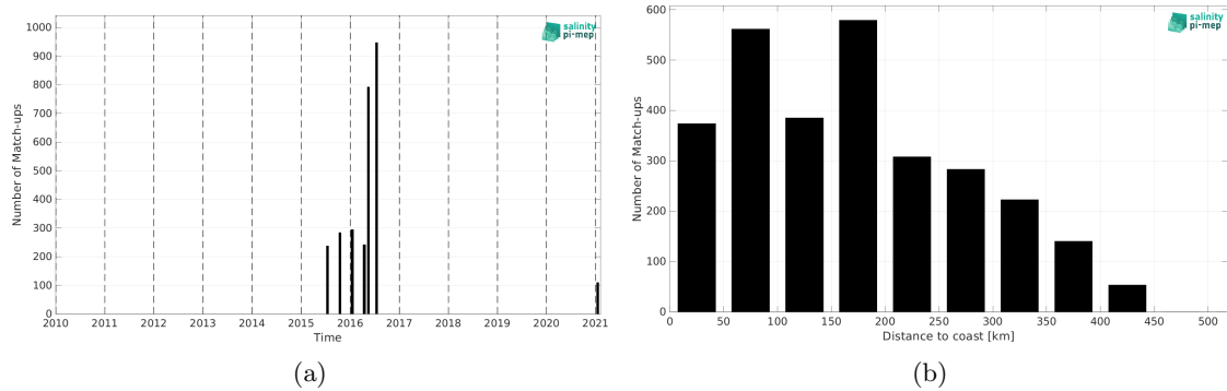
Figure 2: Number of match-ups between TSG (LEGOS-DM) and SMAP SSS L3 v5.0 - 8-Day running (JPL) SSS as a function of time (a) and as function of the distance to coast (b) over the South China Sea Pi-MEP region and for the full satellite product period.
