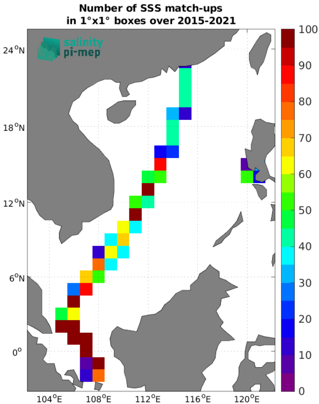
Figure 5: Number of SSS match-ups between TSG (LEGOS-DM) SSS and the SMAP SSS L3 v5.0 - 8-Day running (JPL) SSS product for the South China Sea Pi-MEP region over 1°x1° boxes and for the full satellite product period.
