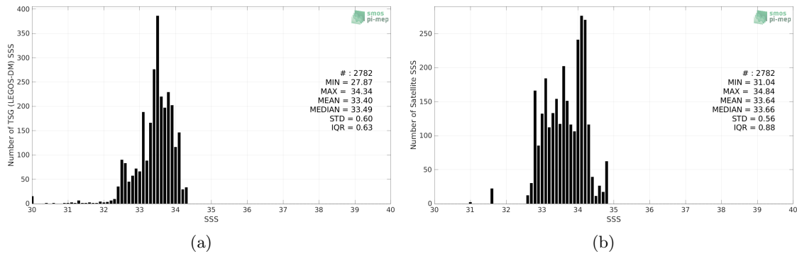
Figure 2: Histograms of SSS from TSG (LEGOS-DM) (a) and SMAP SSS L3 v5.0 - 8-Day running (JPL) (b) considering all match-up pairs per bins of 0.1 over the South China Sea Pi-MEP region and for the full satellite product period.
