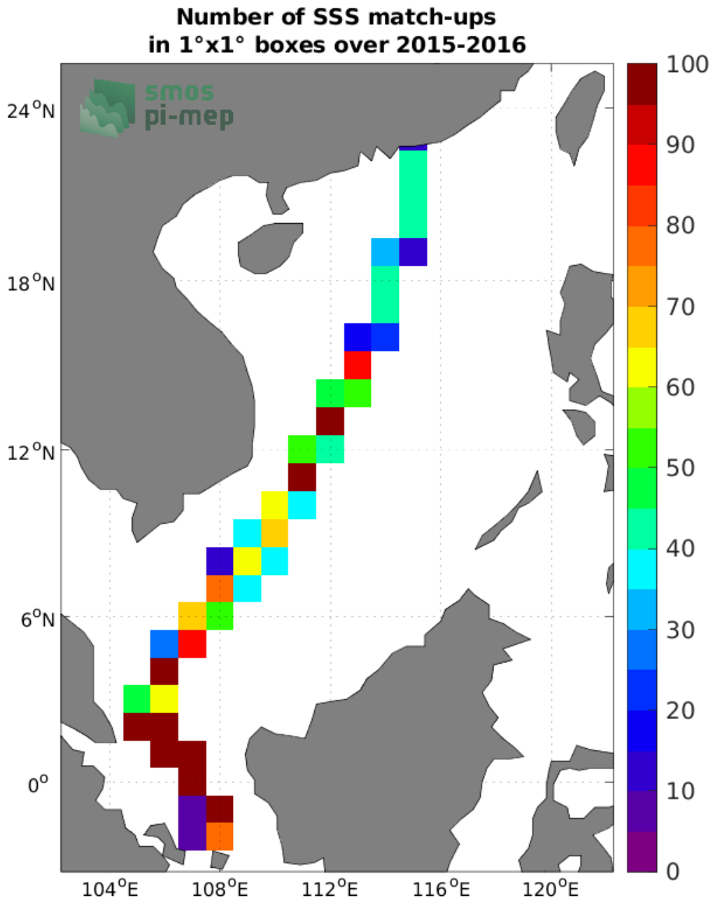
Figure 4: Number of SSS match-ups between TSG (LEGOS-DM) SSS and the SMAP SSS L3 v5.0 - 8-Day running (JPL) SSS product for the South China Sea Pi-MEP region over 1°x1° boxes and for the full satellite product period.
