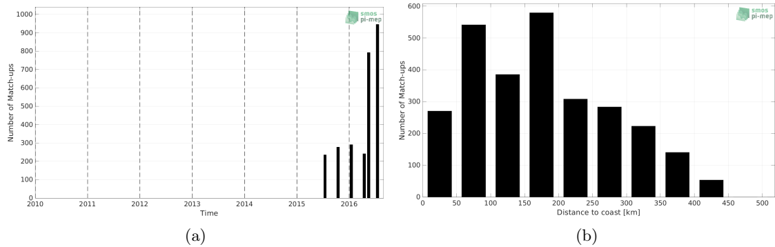
Figure 1: Number of match-ups between TSG (LEGOS-DM) and SMAP SSS L3 v5.0 - 8-Day running (JPL) SSS as a function of time (a) and as function of the distance to coast (b) over the South China Sea Pi-MEP region and for the full satellite product period.
