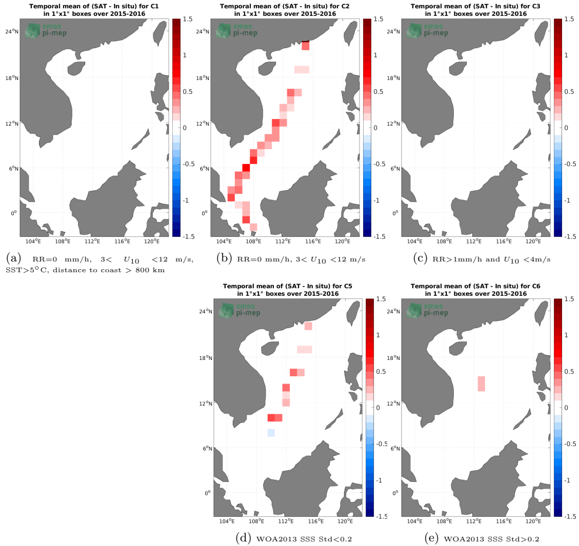
Figure 12: Temporal mean gridded over spatial boxes of size 1^\circ \times 1^\circ of \Delta SSS (SMAP SSS L3 v5.0 - 8-Day running (JPL) - TSG (LEGOS-DM)) for 5 different subdatasets corresponding to: RR=0 mm/h, 3 < U_{10} < 12 m/s, SST > 5°C, distance to coast > 800 km (a), RR=0 mm/h, 3 < U_{10} < 12 m/s (b), RR > 1mm/h and U_{10} < 4 m/s (c), WOA2013 SSS Std < 0.2 (d), WOA2013 SSS Std > 0.2 (e).
